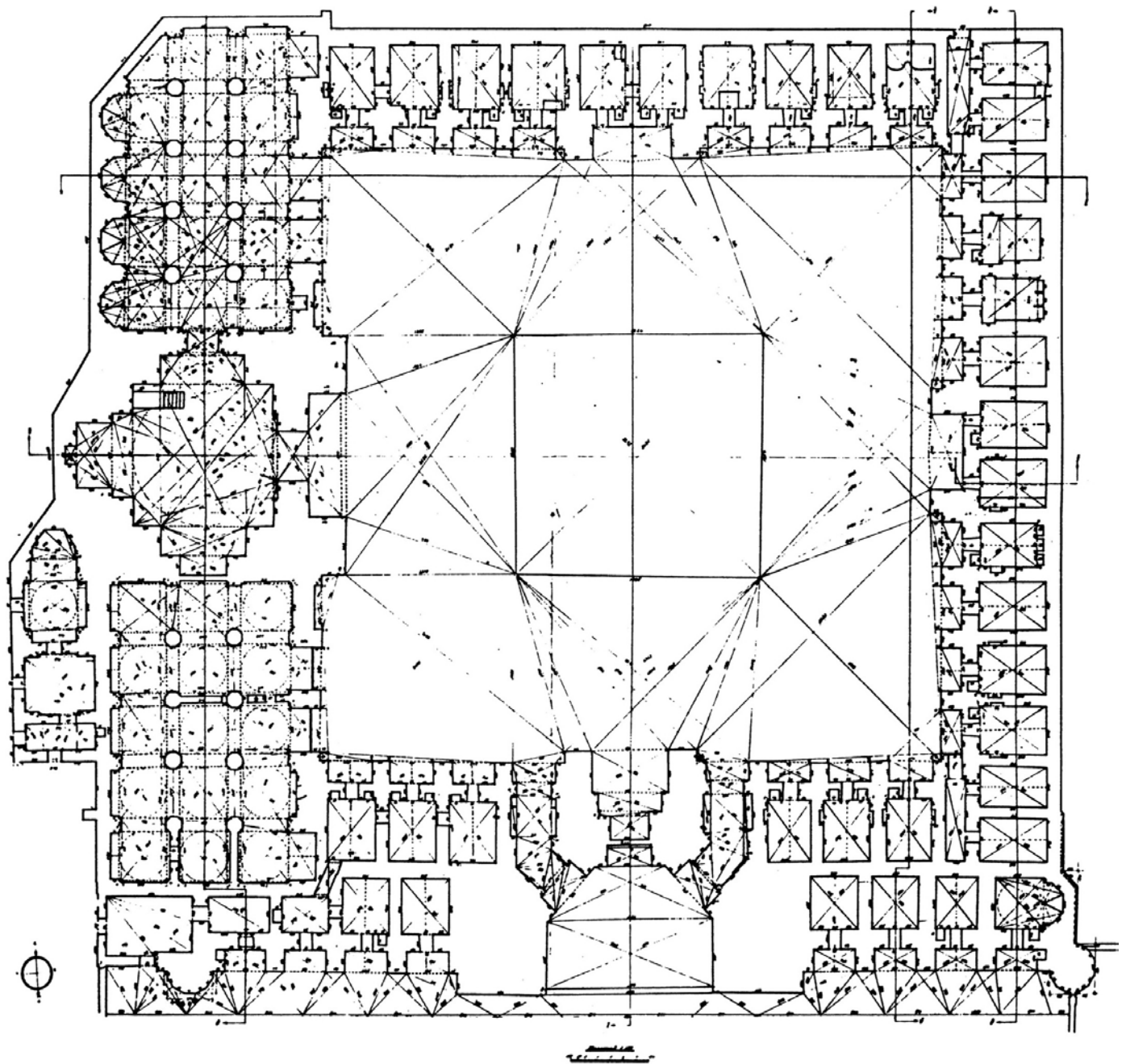
Tillya Kari madrasa and mosque, ground floor plan
