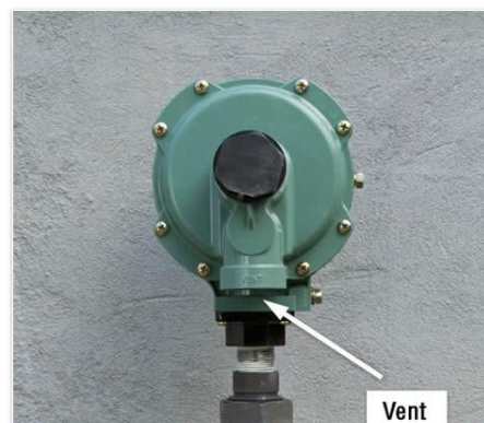
#3 Regulator on side of house, showing vent. Vent needs to be clear of snow and ice.
