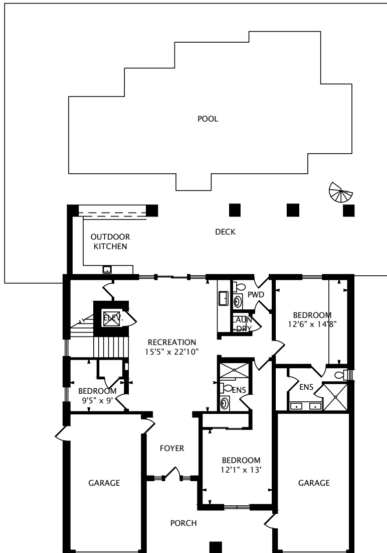
MAIN FLOOR 1555 SQUARE FEET
