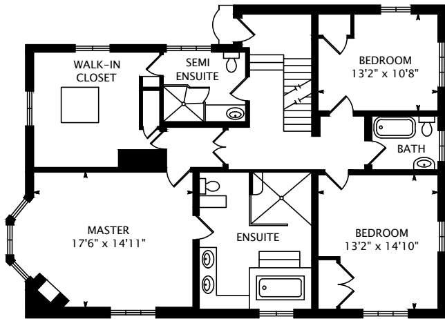
SECOND FLOOR 1503 SQUARE FEET
