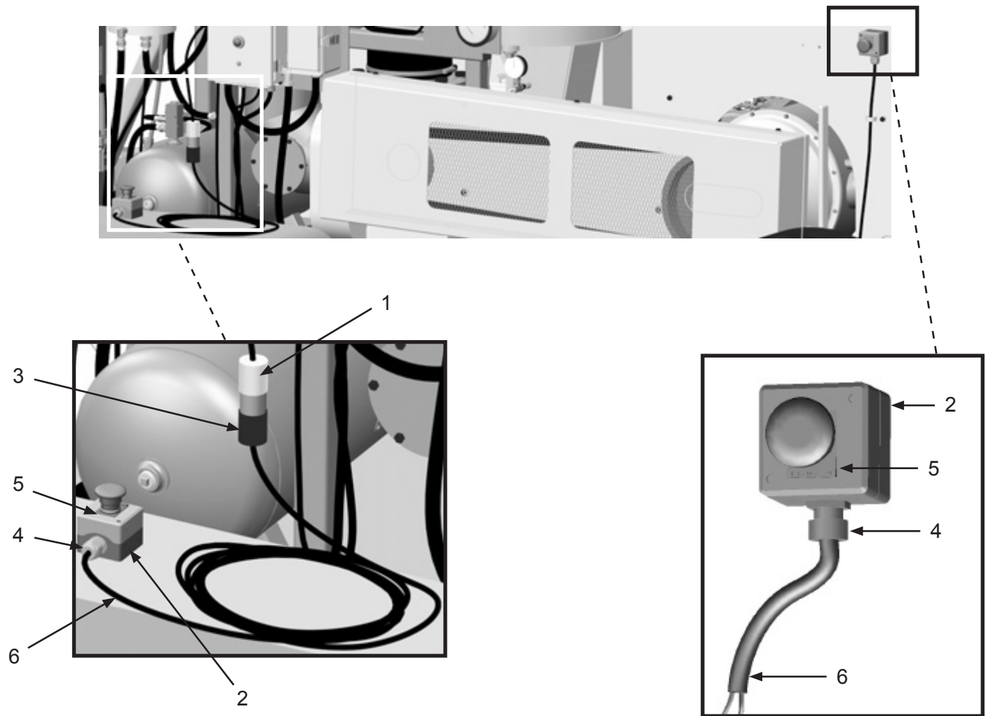
Figure 17: Emergency-Stop Stations
