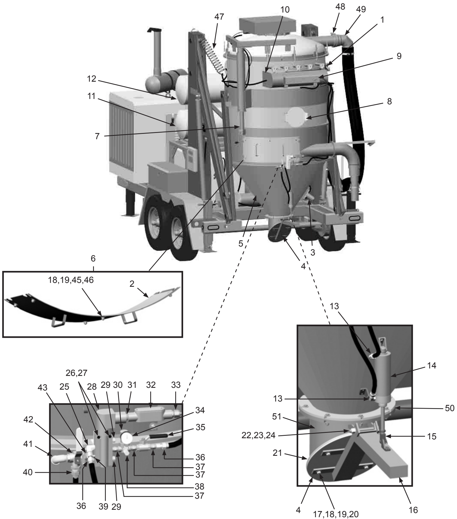
Figure 2: Rear Assembly
