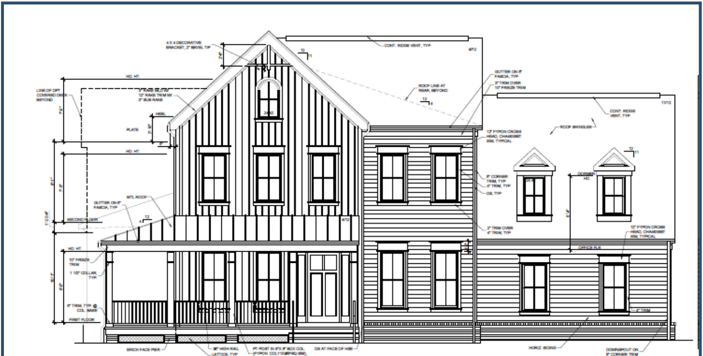
Draft front elevation of house being built on Lot 3. Construction commenced May 2017
