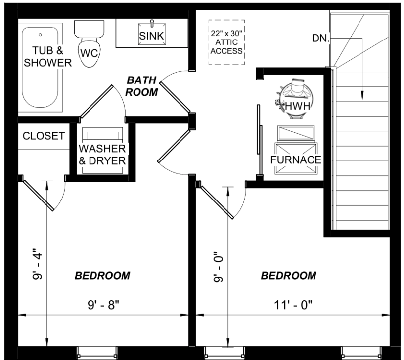
THIRD FLOOR 438 Sq. Ft.
