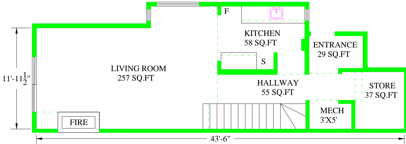
1 MAIN FLOOR PLAN Scale: 3/16" TO 1'
