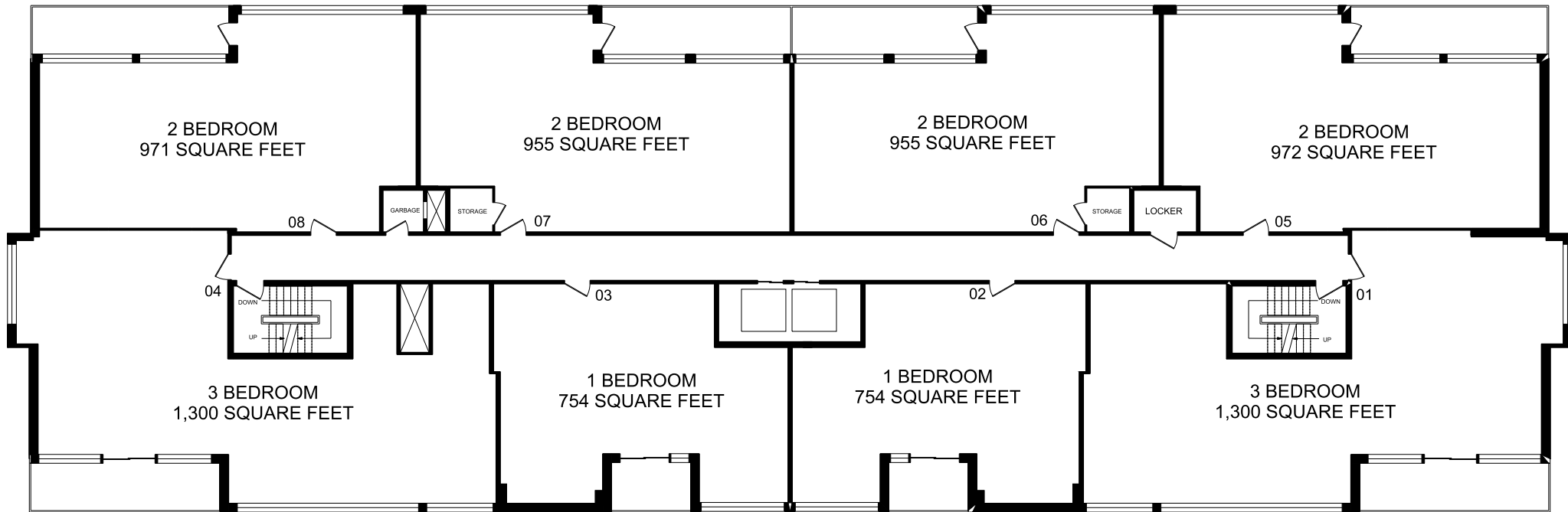
205 QUEEN MARY DRIVE TYPICAL FLOOR
