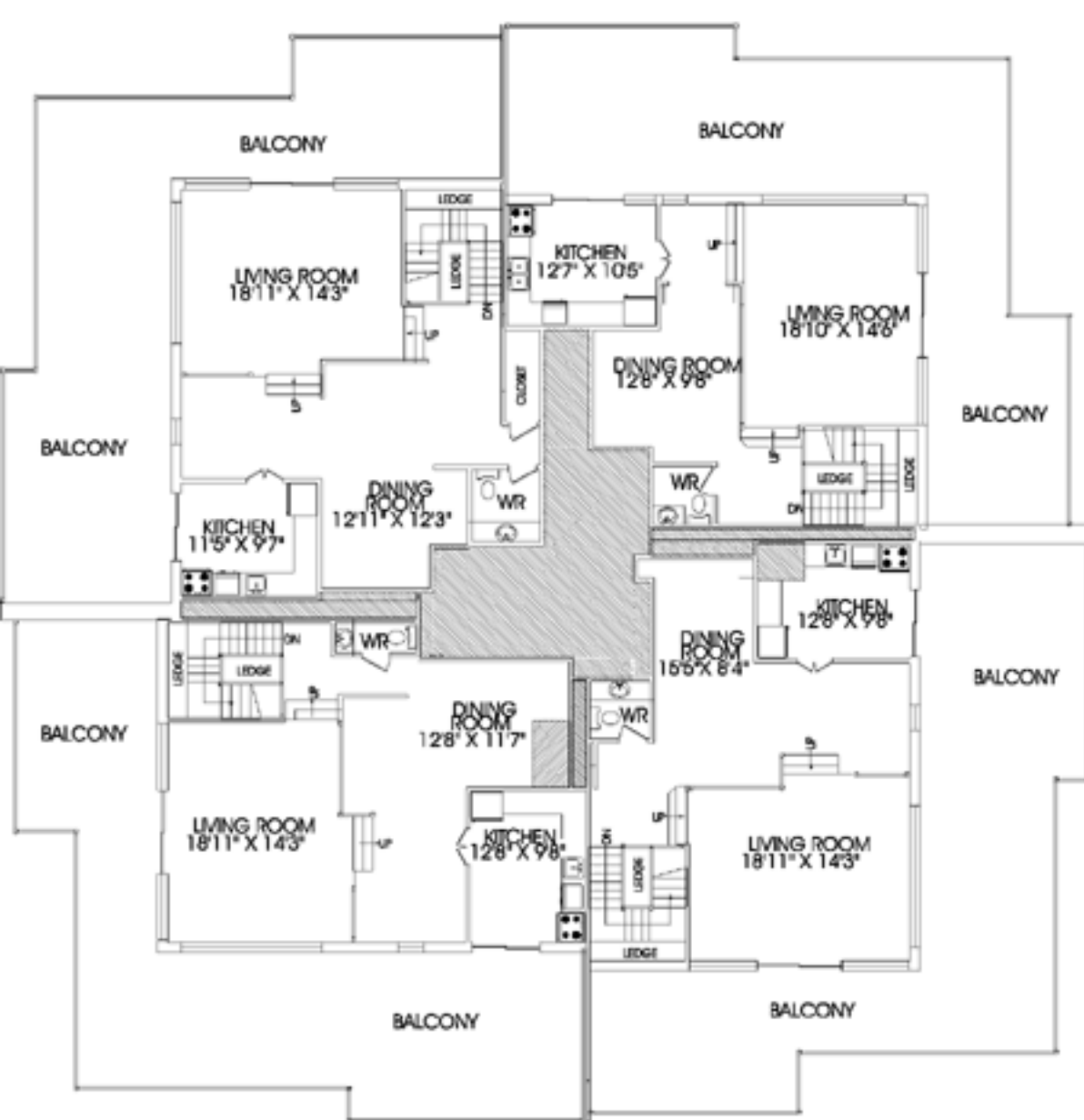
PENTHOUSE SECOND FLOOR
