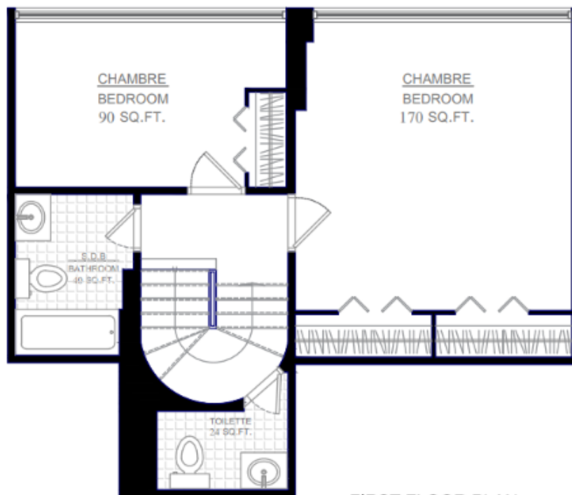
FIRST FLOOR PLAN TOTAL AREA: 490 SQ. FT.
