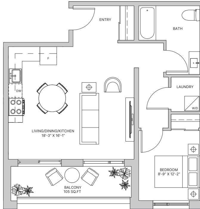
LEVELS 2-9
