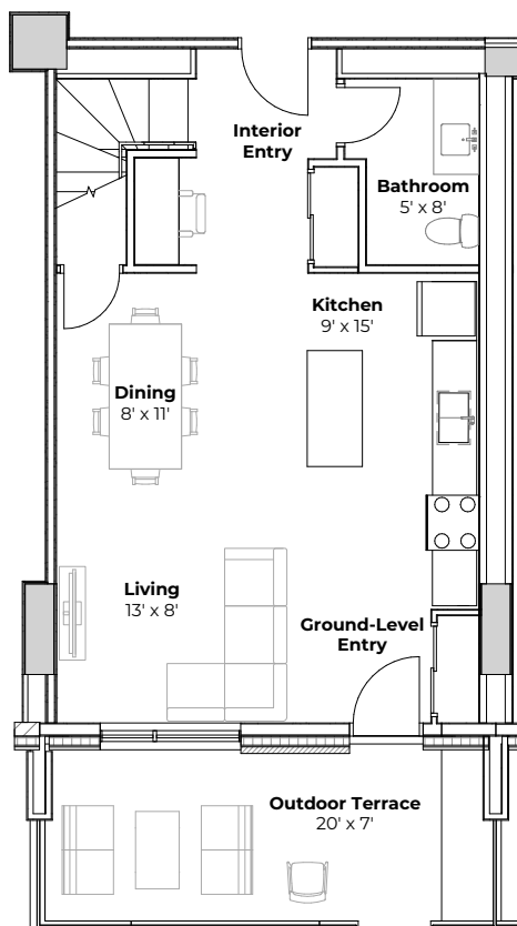
LEVEL ONE Living/Kitchen/Dining 557 Square Feet
