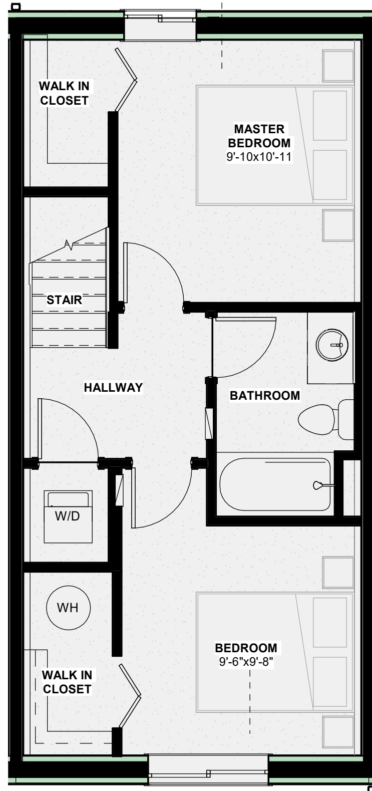
1 TYPICAL LOWER SUITE PLAN BASEMENT 1/4" = 1'-0"
