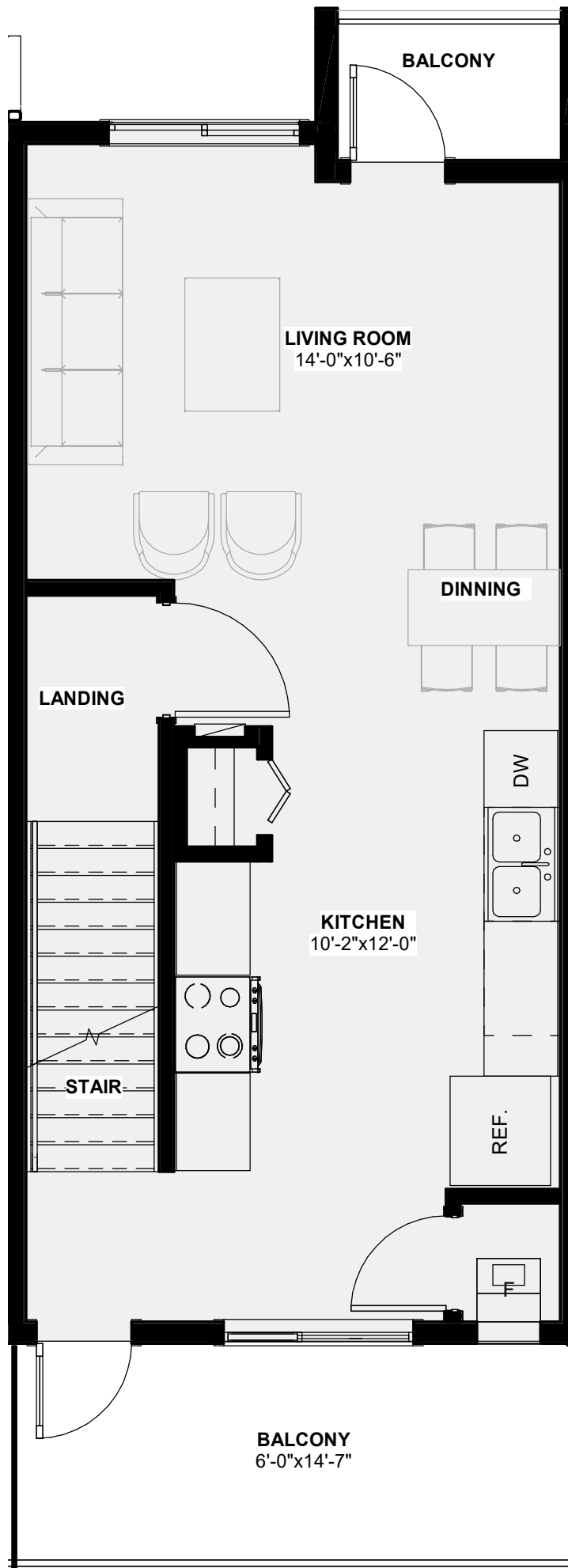
2 UPPER TYP. SUITE SECOND FLOOR PLAN ADV-02 1/4" = 1'-0"
