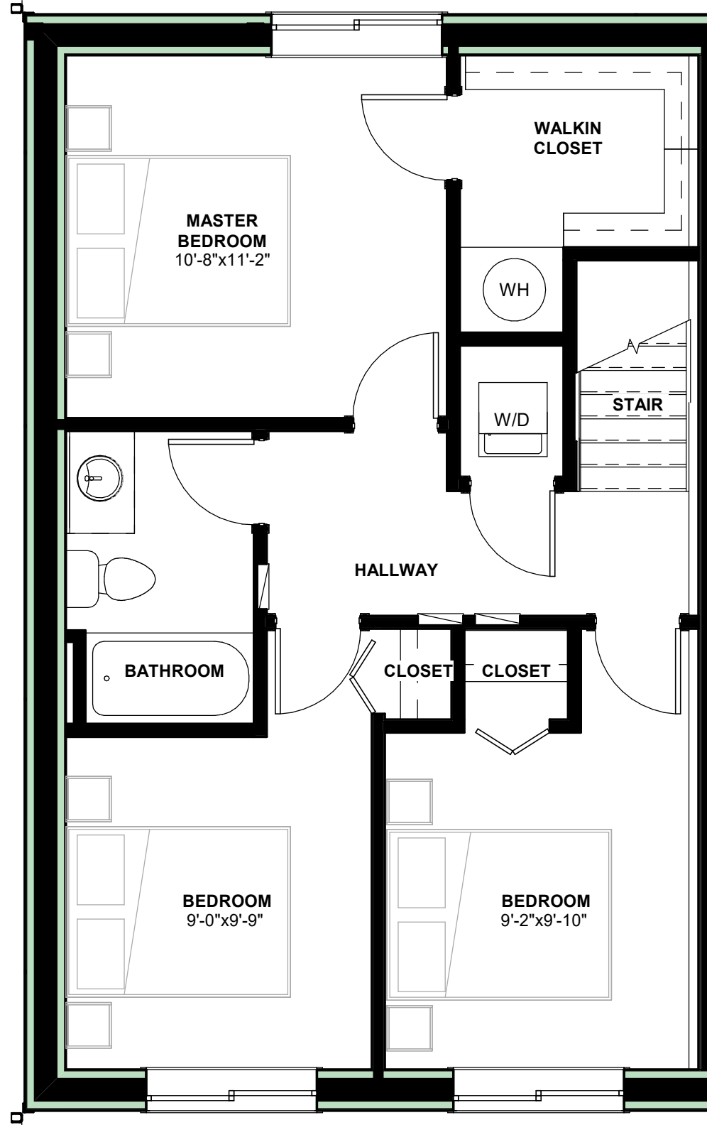
1 WEST END LOWER SUITE BASEMENT PLAN A5.1/ADV-03 1/4" = 1'-0"
