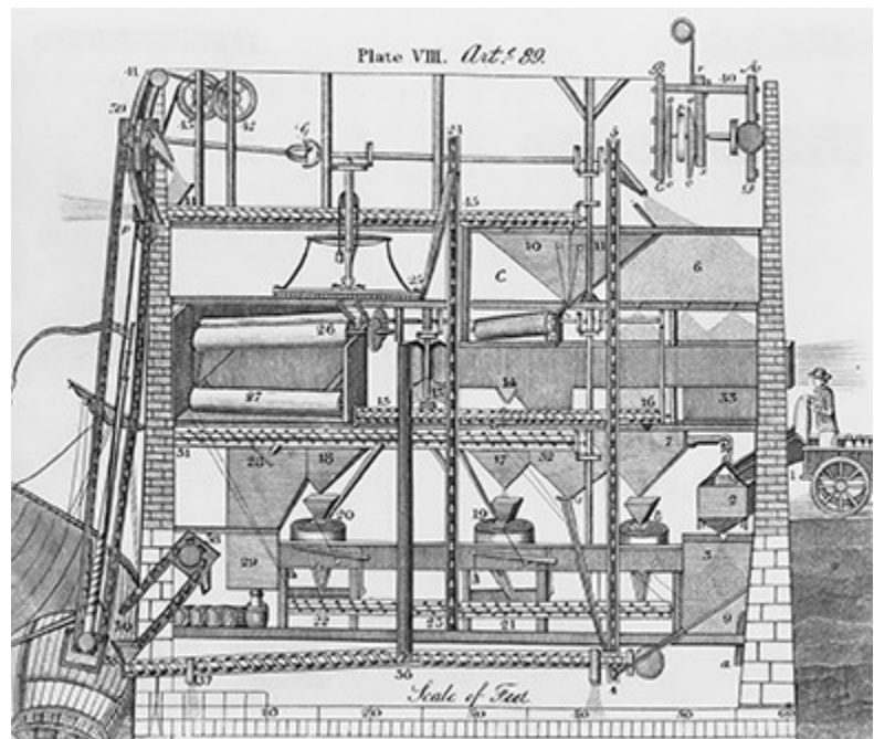
Oliver Evans was an American engineer and inventor, best known for developing ways to automate the flour milling process, which is illustrated
