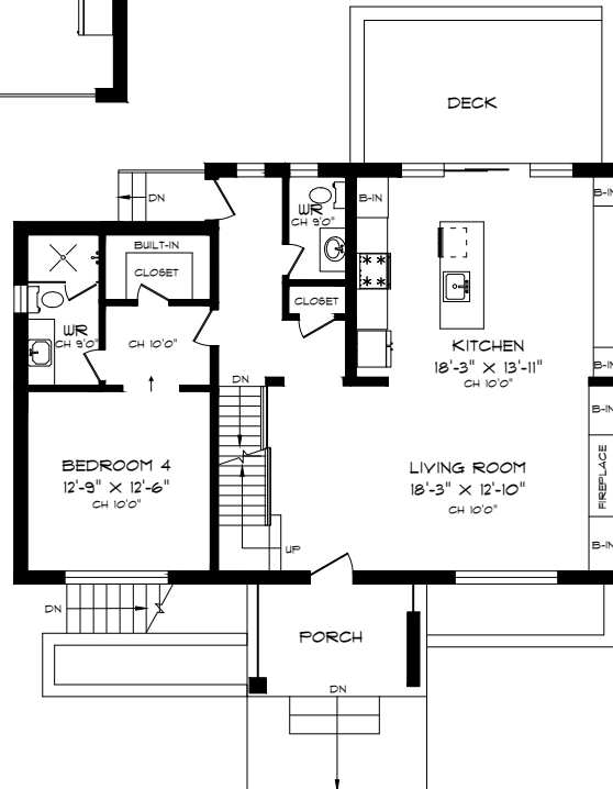
MAIN FLOOR 1,202 SQUARE FEET
