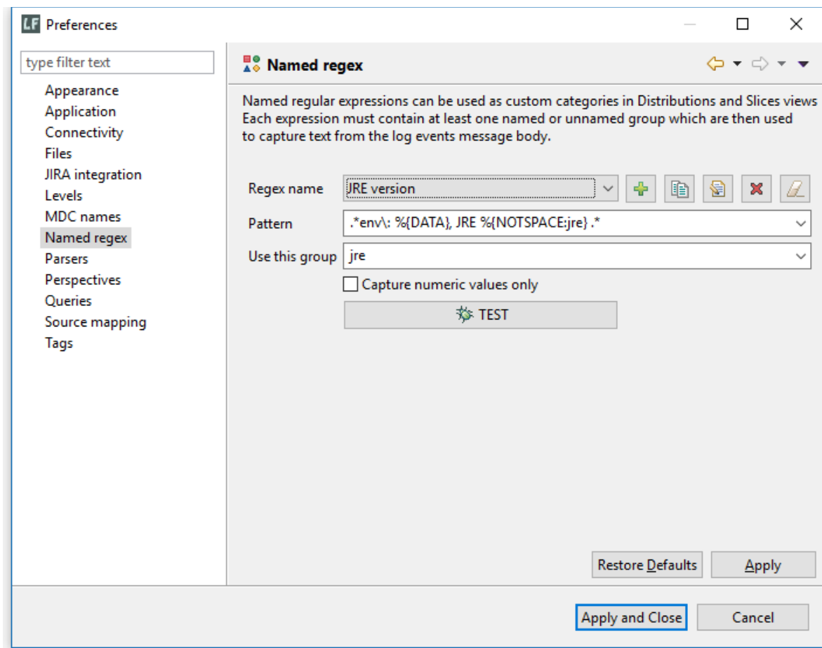
Figure 3.18.8
