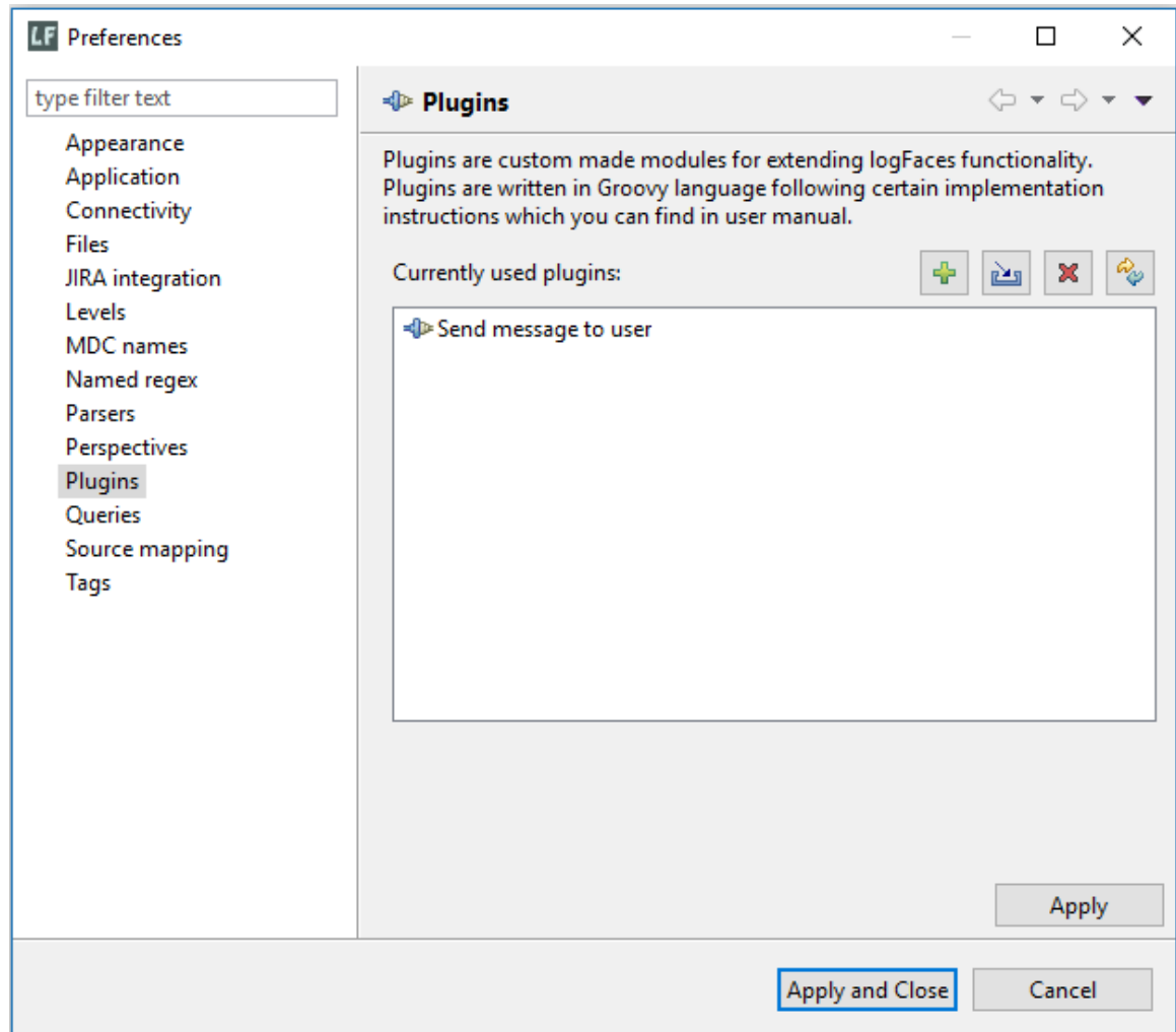
Figure 3.18.11: Plugins management
