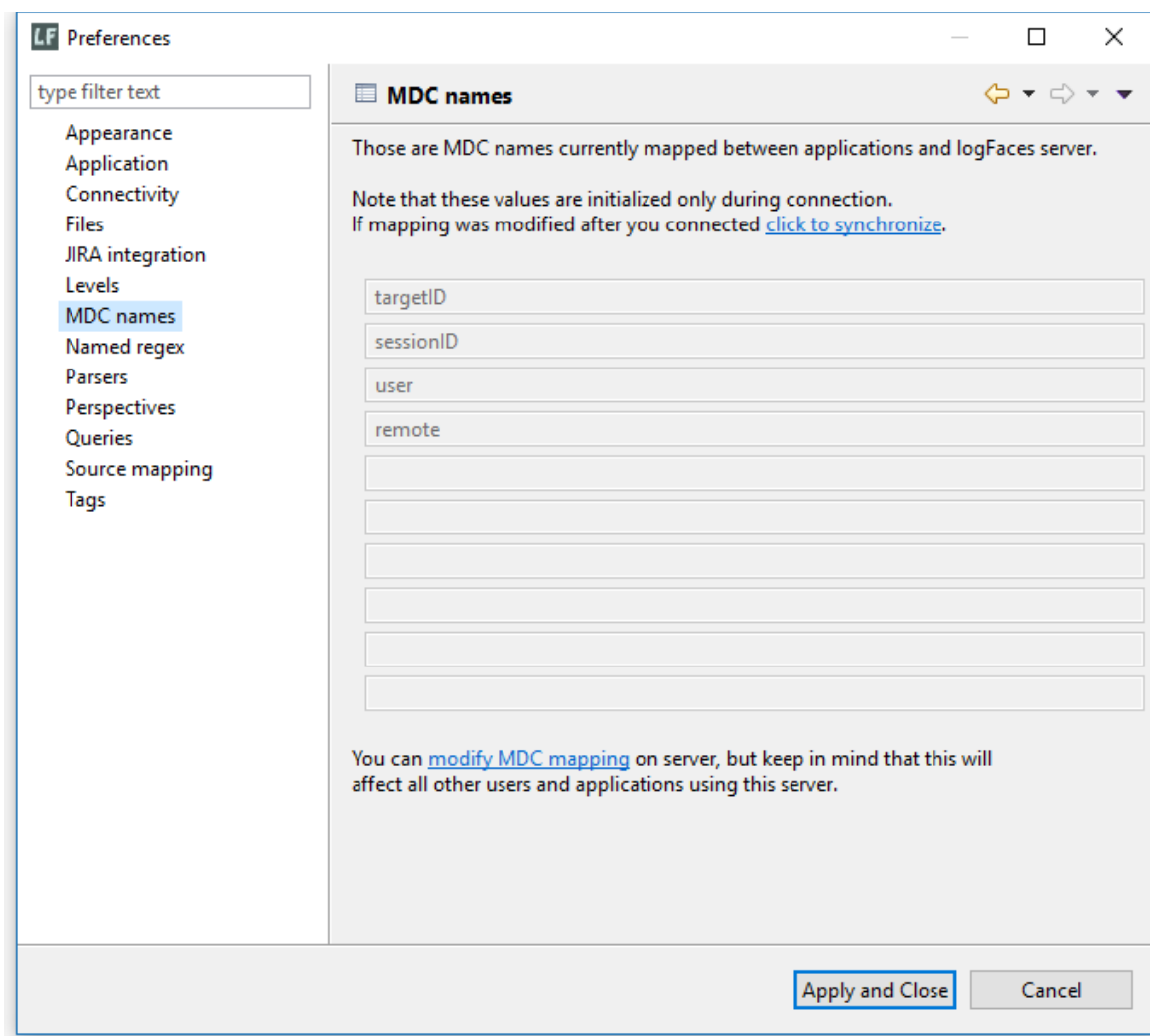
Figure 3.18.7: MDC mapping
