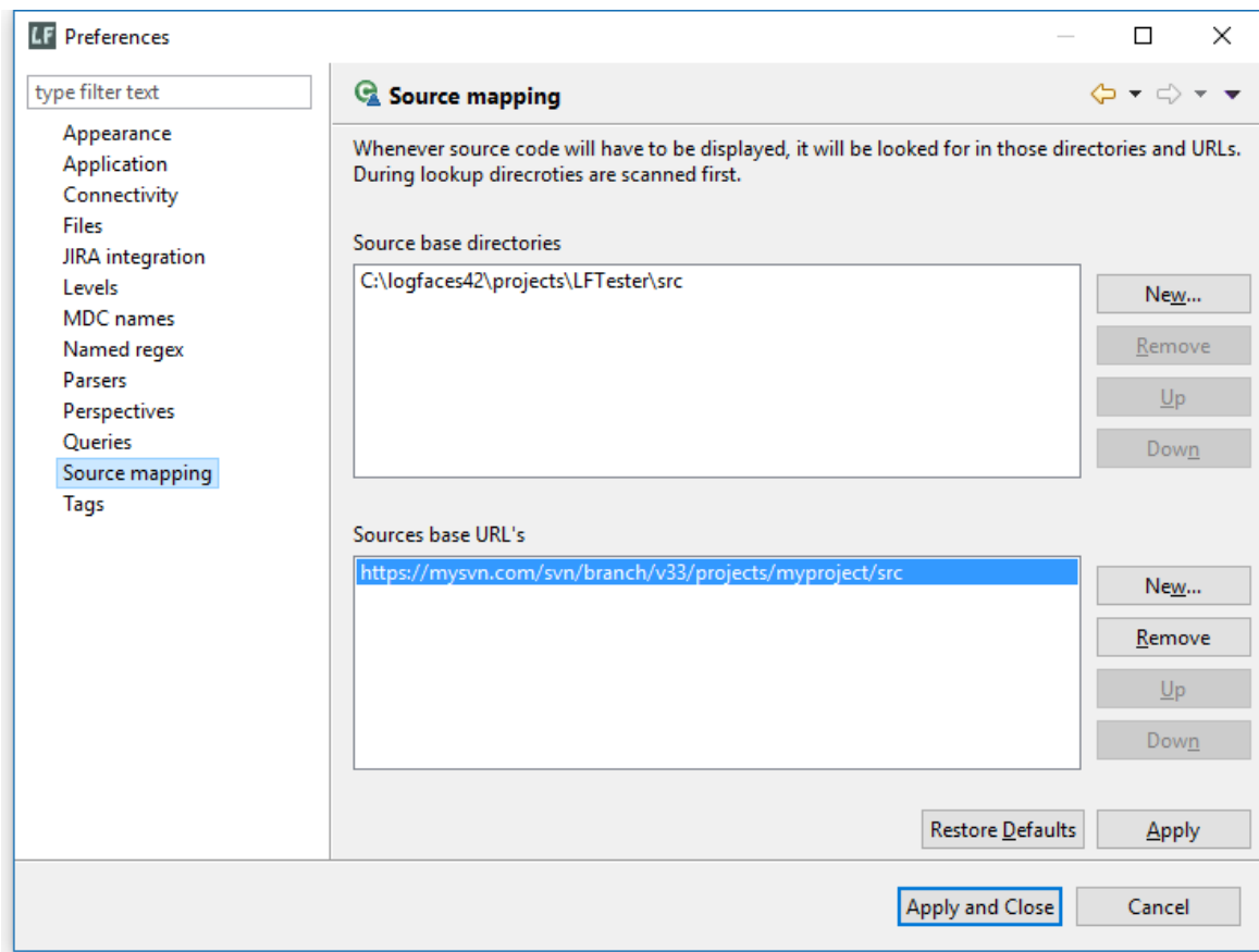
Figure 3.18.13: Sources mapping
