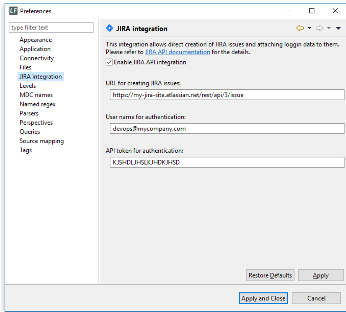
Figure 3.18.5: JIRA integration
