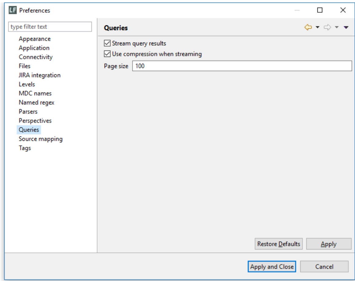
Figure 3.18.12: Query preferences
