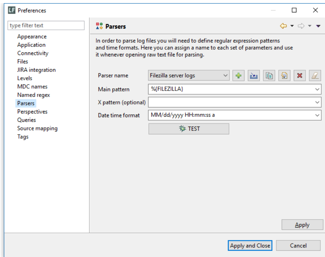
Figure 3.18.9: Parsers
