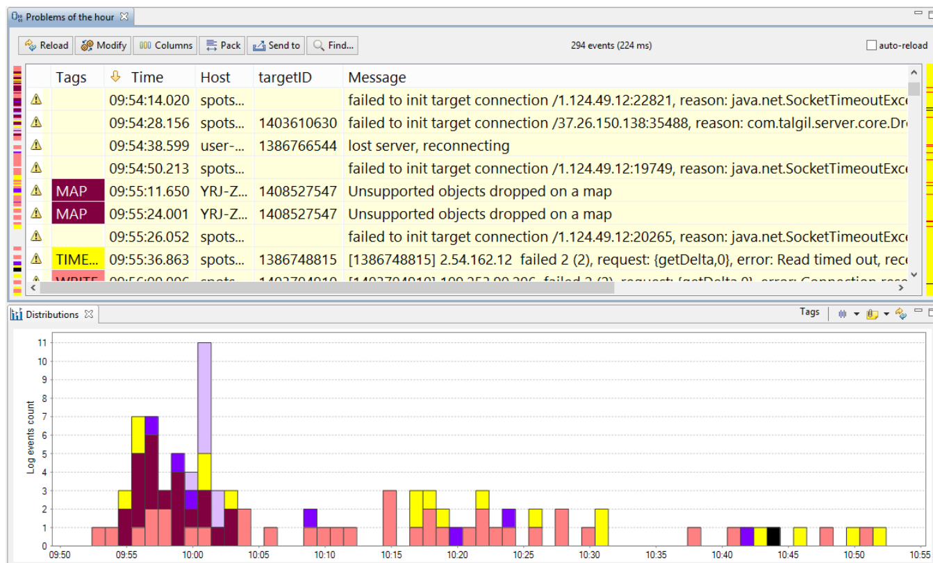
Figure 3.9.6: Distributions example
