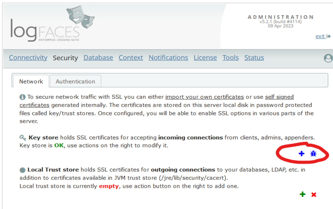
Figure 2.9.10: SSL setup
