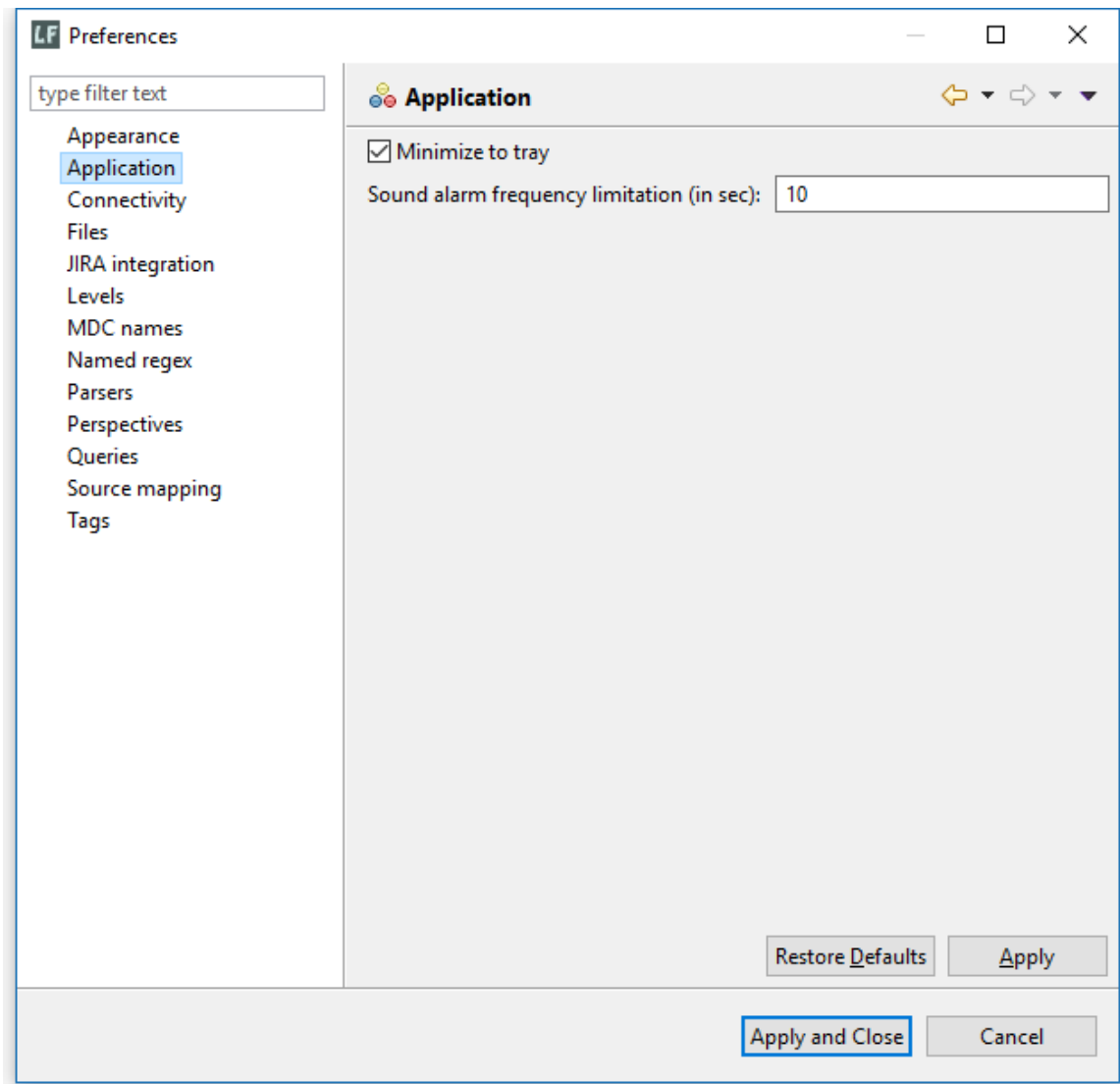
Figure 3.18.2: Application preferences
