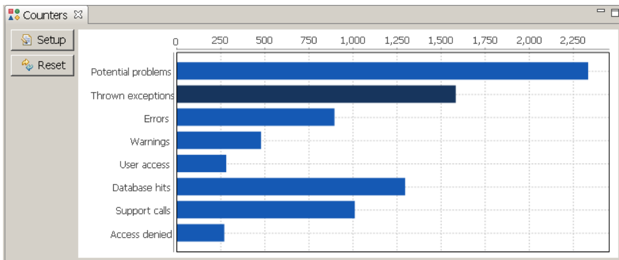
Figure 3.9.13: Counters view
