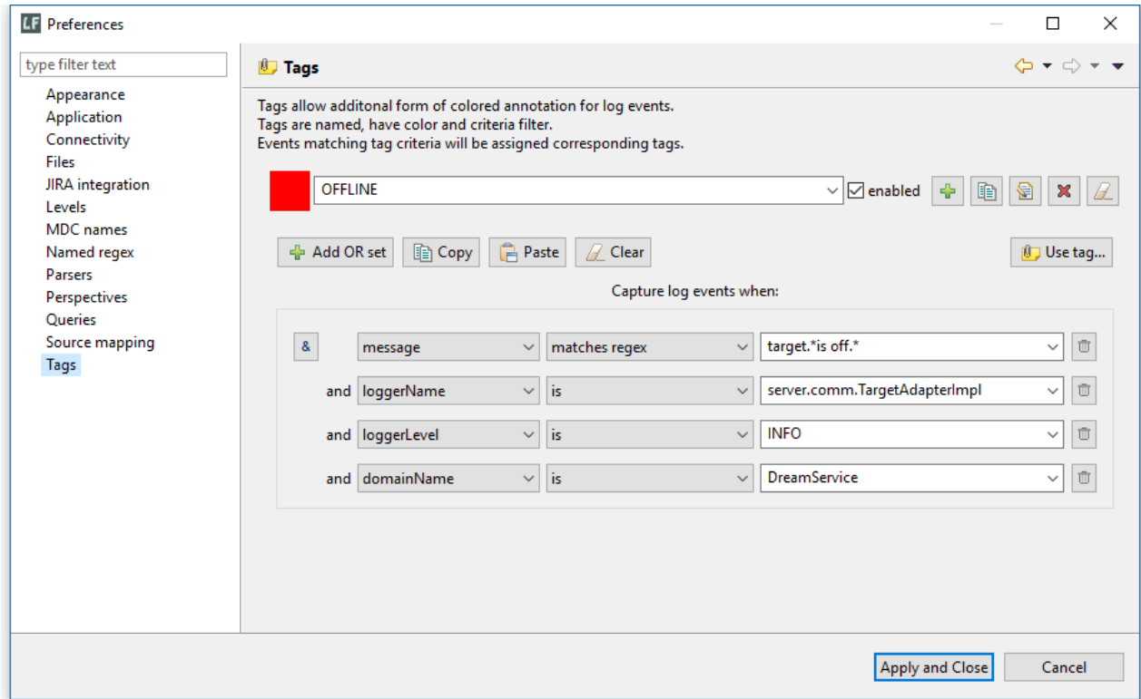
Figure 3.18.14: Tags preferences
