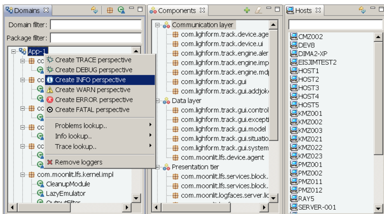
Figure 3.10.1: Repositories
