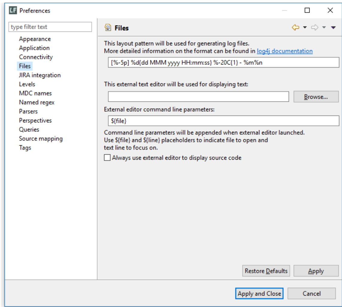
Figure 3.18.4: File preferences
