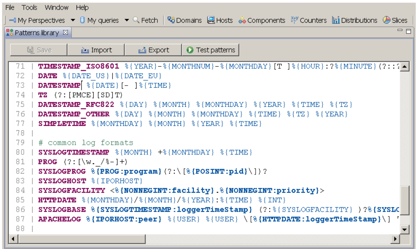
Figure 3.14.1: Patterns library
