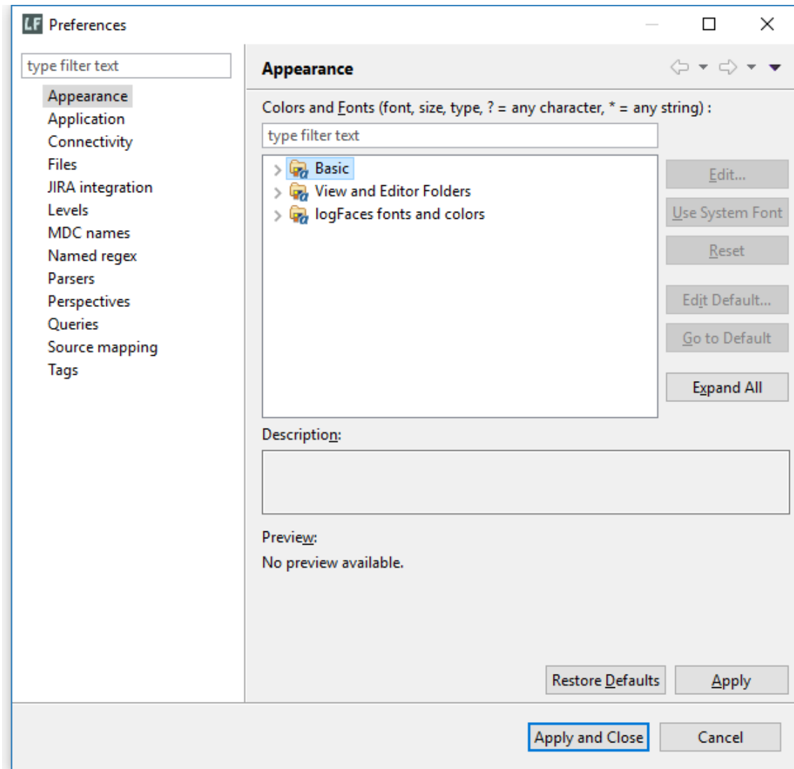
Figure 3.18.1: Appearance
