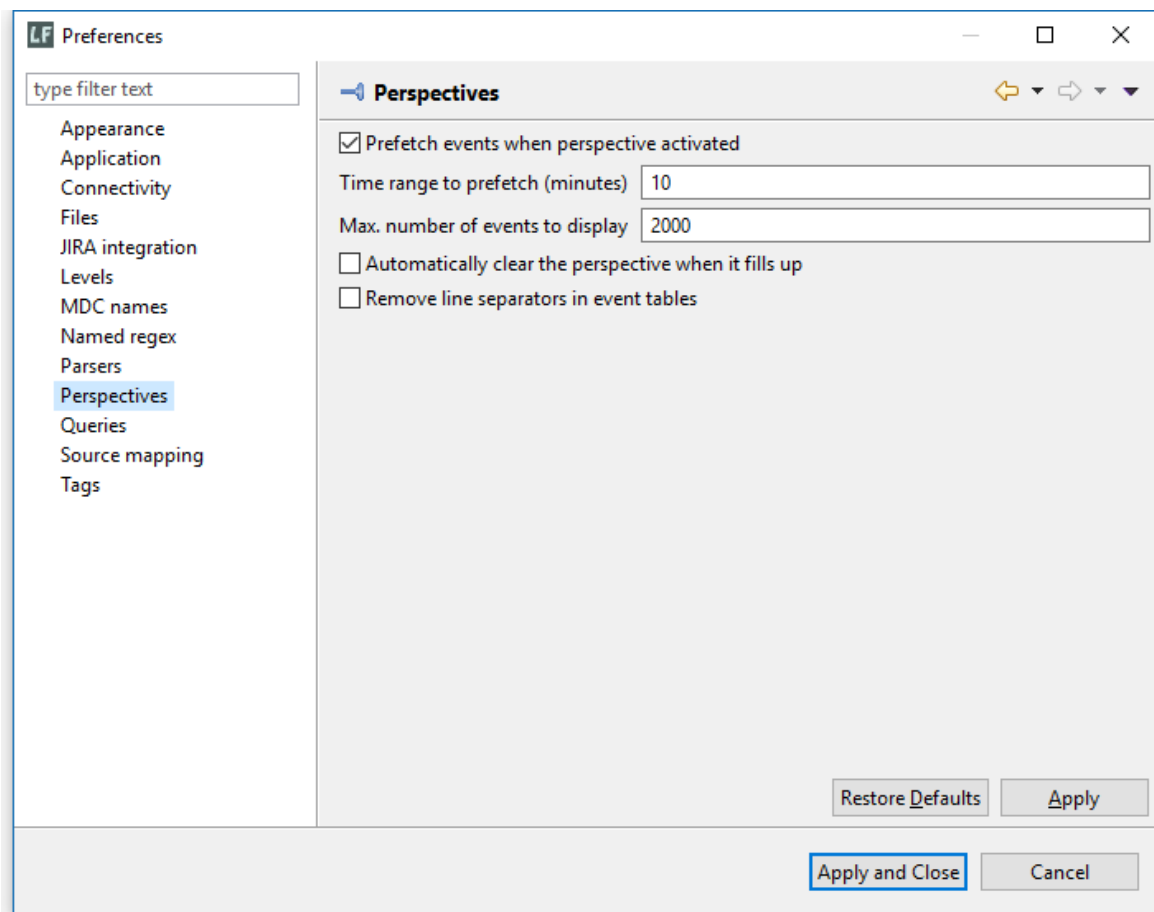
Figure 3.18.10: Perspective preferences
