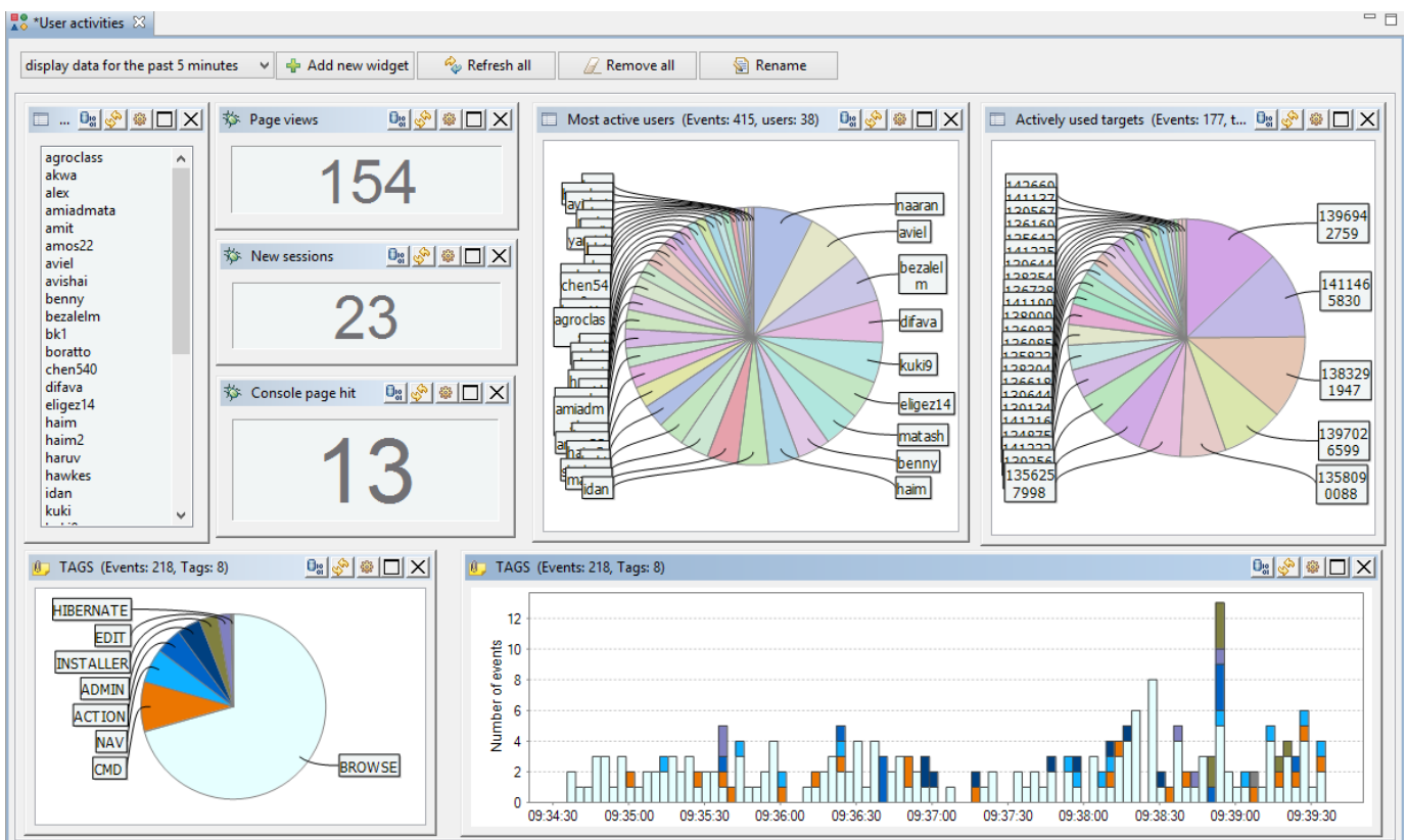
Figure 3.9.1: Dashboard example
