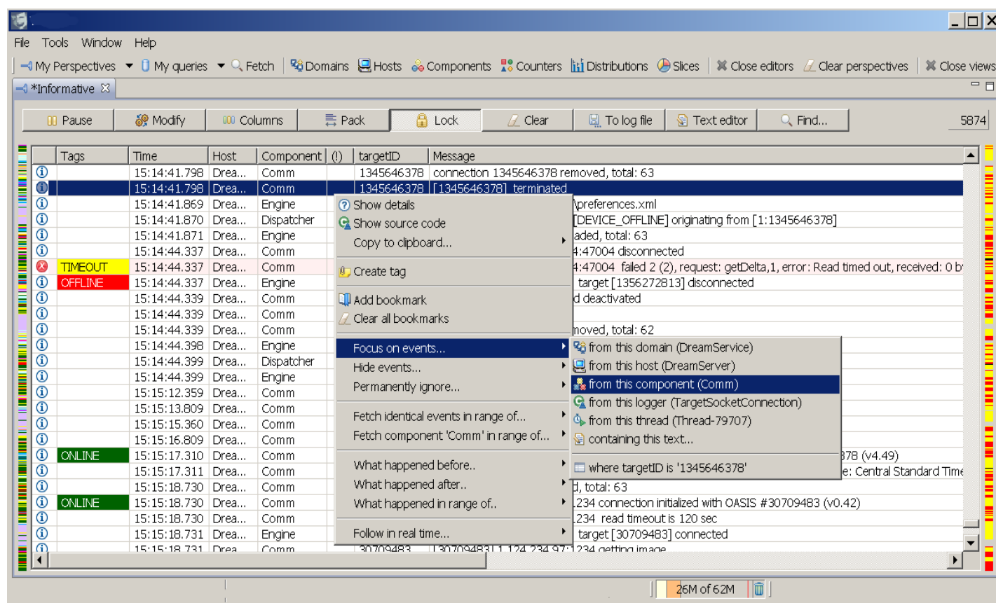
Figure 3.5.1: Data tables
