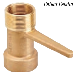
1 1/2" MPT x 1 1/4" FPT outlet 1 1/2" FPT inlet
