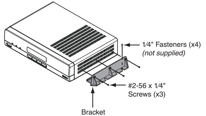
Figure 13: Interface Box Mounting
