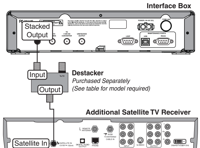
Figure 11: Connecting an Additional Receiver
