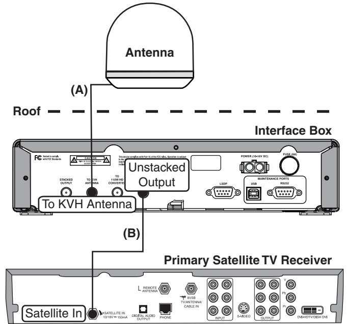
Figure 9: Wiring the Interface Box
