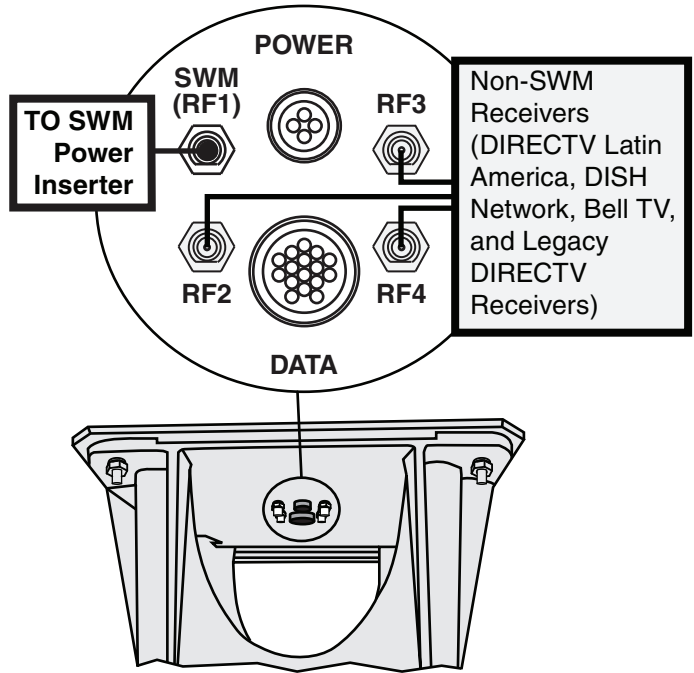
Figure 11 Connectors on Bottom of Antenna Assembly
