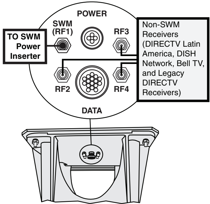
Figure 12 Connectors on Bottom of Antenna Assembly
