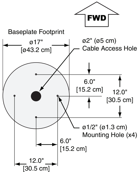
Figure 7 Antenna Mounting Holes Layout
