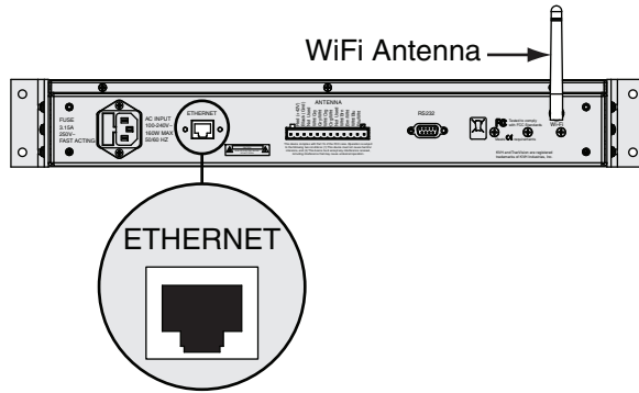
Figure 32 Connection Options
