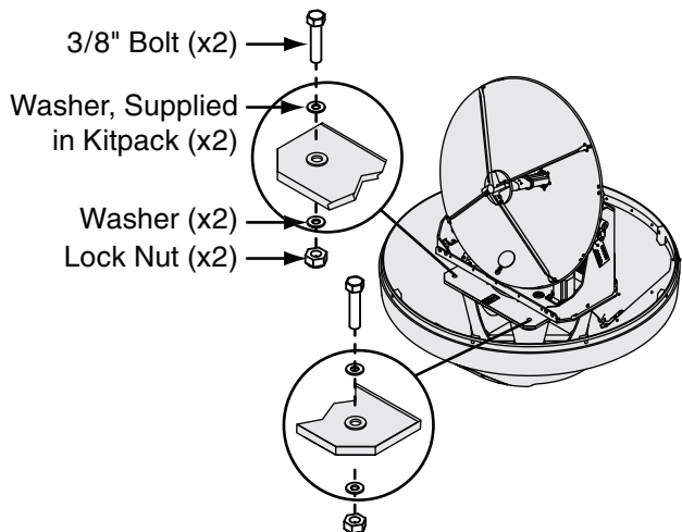
Figure 16 Mounting Bolt Reinstallation
