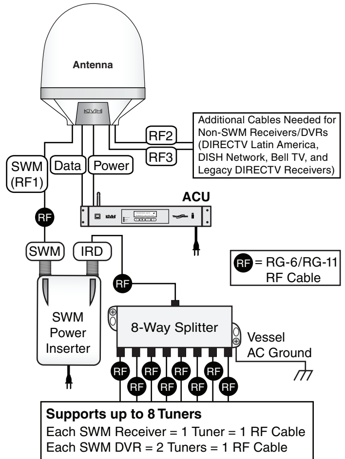
Figure 6 Wiring Overview
