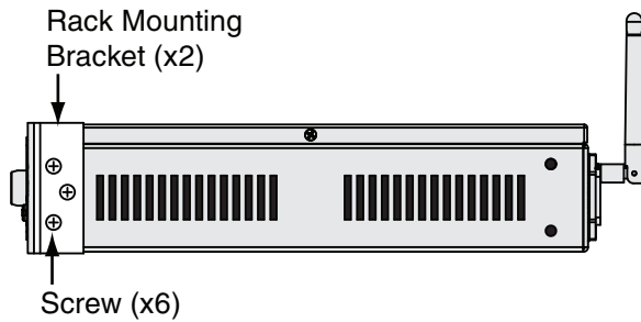
Figure 19 ACU Rack Mounting Bracket Removal
