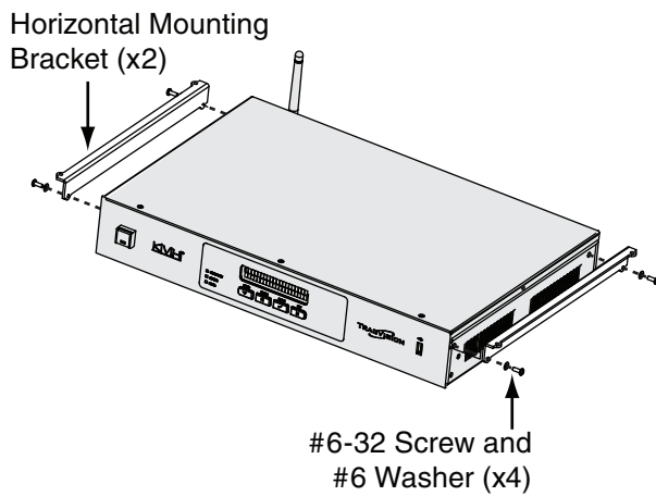
Figure 20 Horizontal Mounting Bracket Orientation
