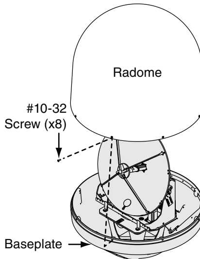
Figure 10 Radome Screws
