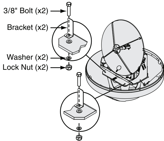
Figure 15 Shipping Restraint Bracket Removal
