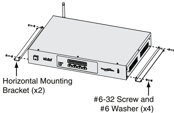
Figure 21 Horizontal Mounting Bracket Orientation
