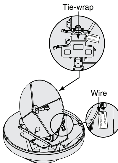
Figure 17 Shipping Restraints
