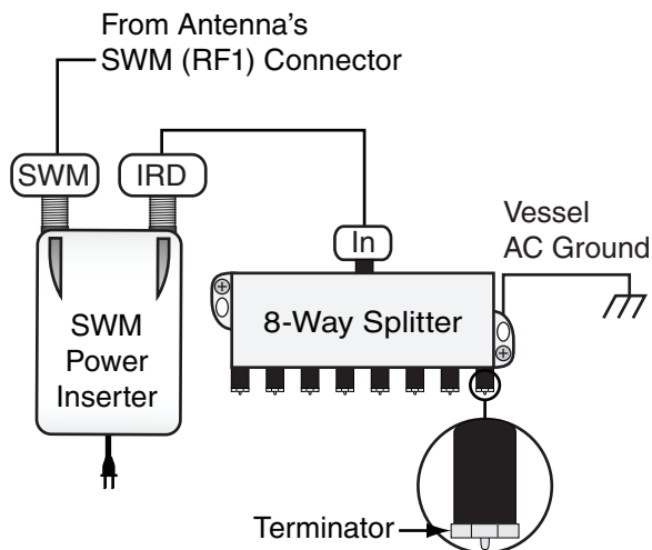
Figure 26 8-Way Splitter Connection (DIRECTV Only)
