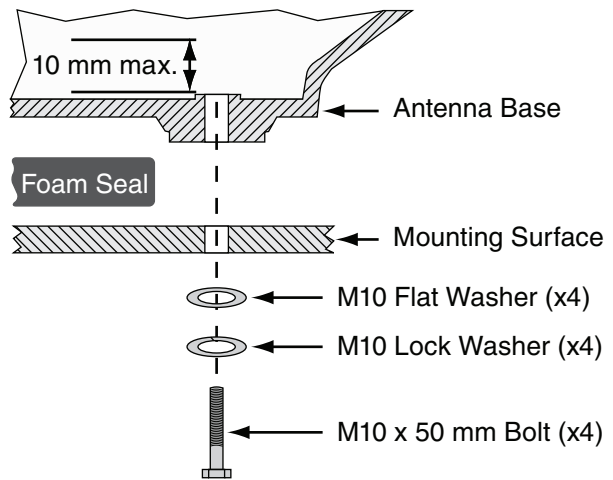
Figure 14 Antenna Mounting
