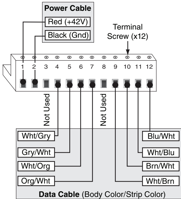
Figure 22 Terminal Strip Connector
