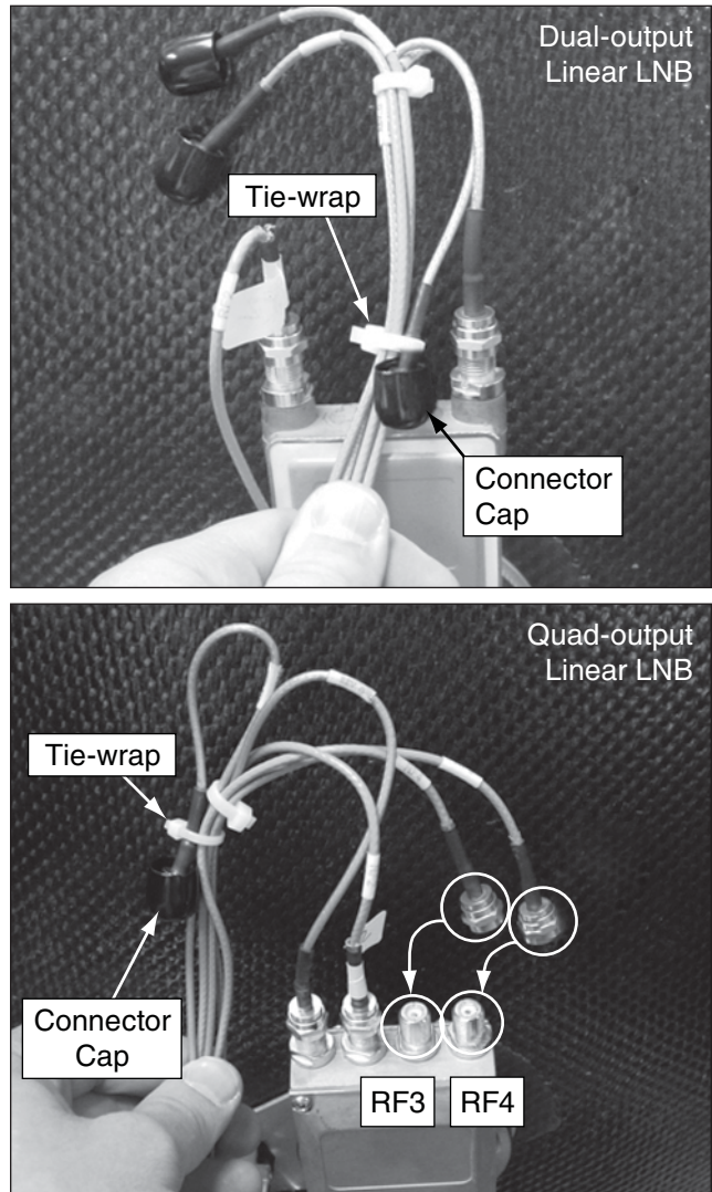
Figure 36 Cable Connections/Tie-wrap
