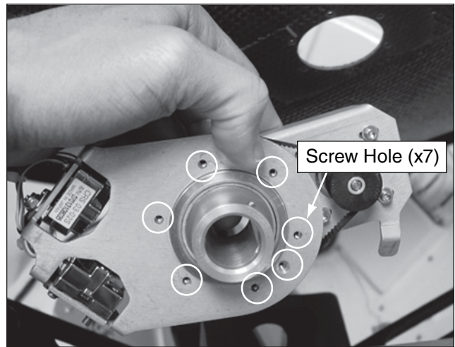
Figure 22 Screw Hole Alignment
