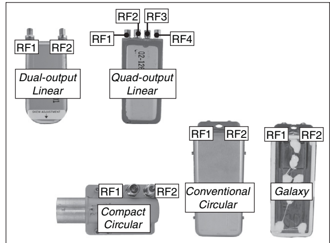
Figure 51 LNB Cable Connections
