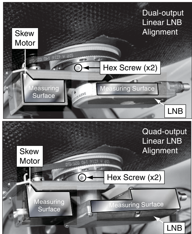
Figure 32 LNB Alignment
