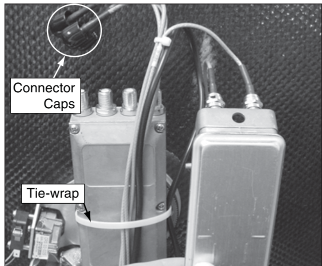
Figure 59 RF Cables/Connector Caps/Tie-wrap
