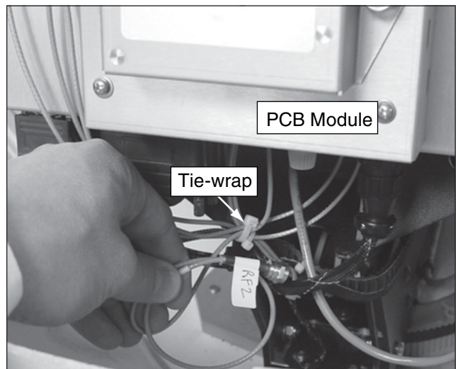
Figure 7 RF Cable/Tie-wrap
