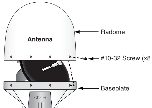
Figure 1 TracVision M9 Radome Screws
