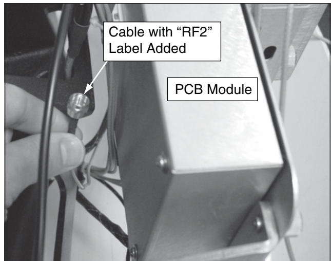
Figure 18 Cable Routing
