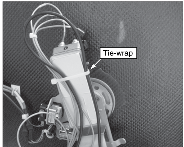
Figure 54 Galaxy/Conventional Circular LNB Tie-wrap Location
