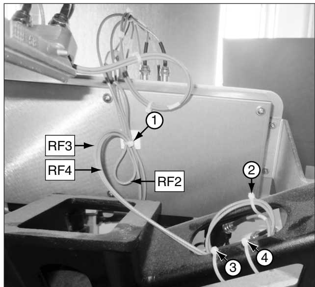
Figure 56 RF2, RF3, and RF4 Cable Loops and Tie-wraps
