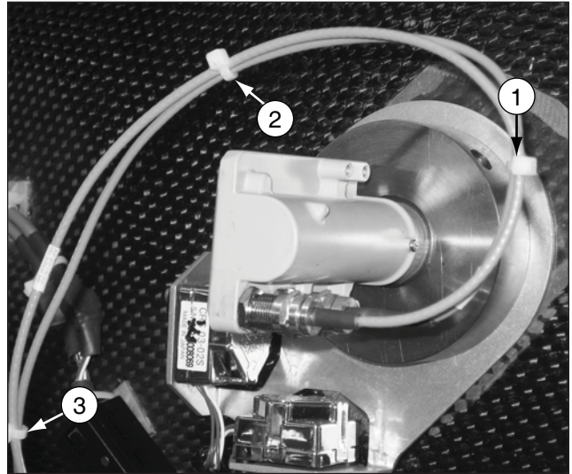
Figure 62 Compact Circular Tie-wrap Locations
