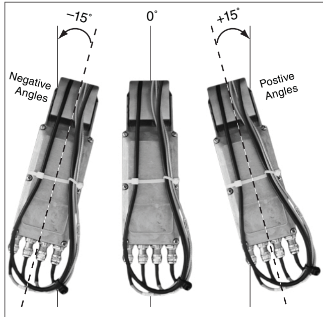
Figure 34 Positive/Negative Skew Angles
