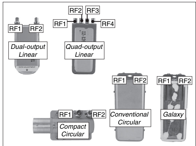
Figure 58 LNB Cable Connections
