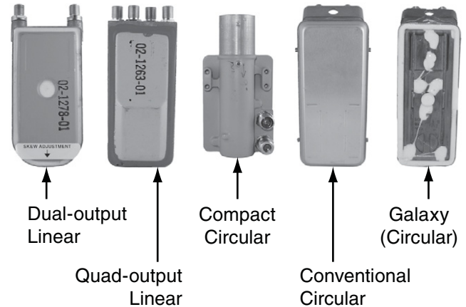
Figure 2 LNB Types
