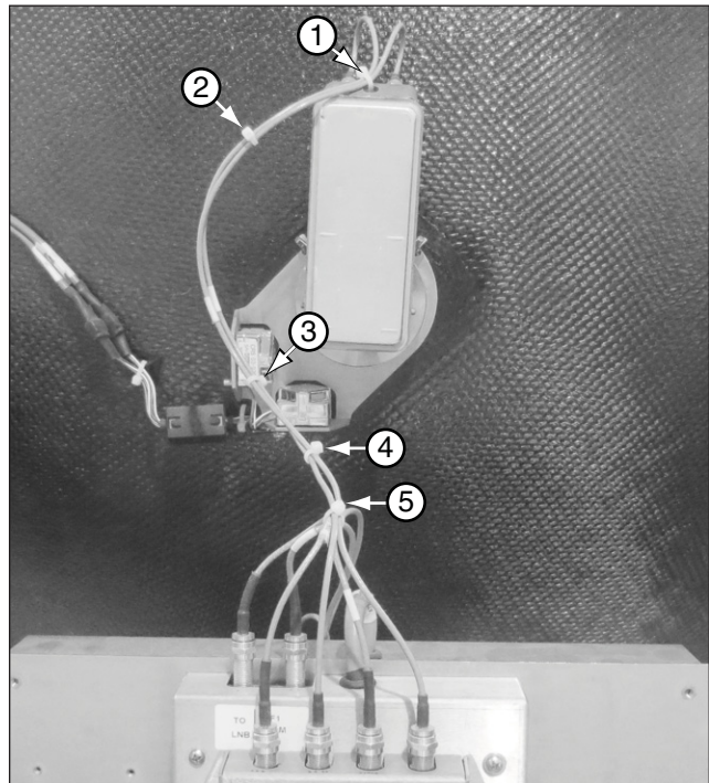
Figure 55 RF2 to "RF2 FROM IRD" Connector and Tie-Wraps
