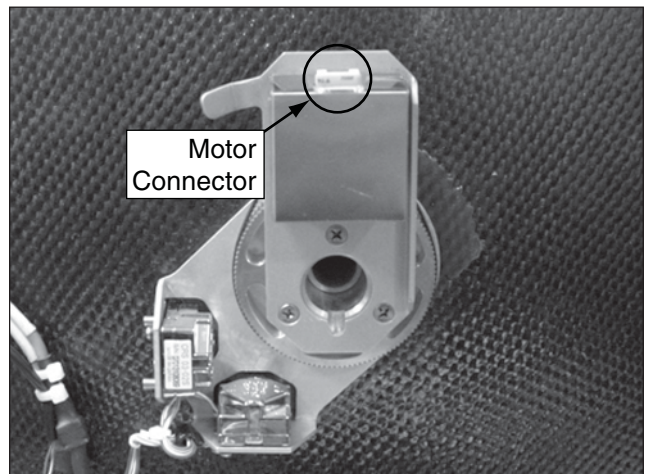
Figure 27 Motor Connector
