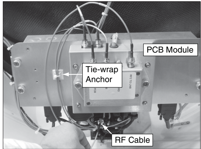
Figure 17 "RF2 TO LNB" Cable Routing
