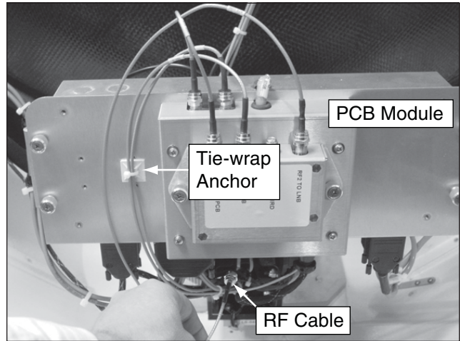
Figure 8 Cable Routing
