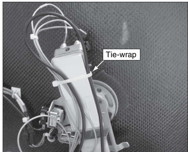
Figure 61 Galaxy/Conventional Circular LNB Tie-wrap Location
