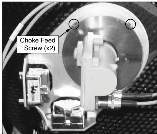
Figure 60 Choke Feed Screws
