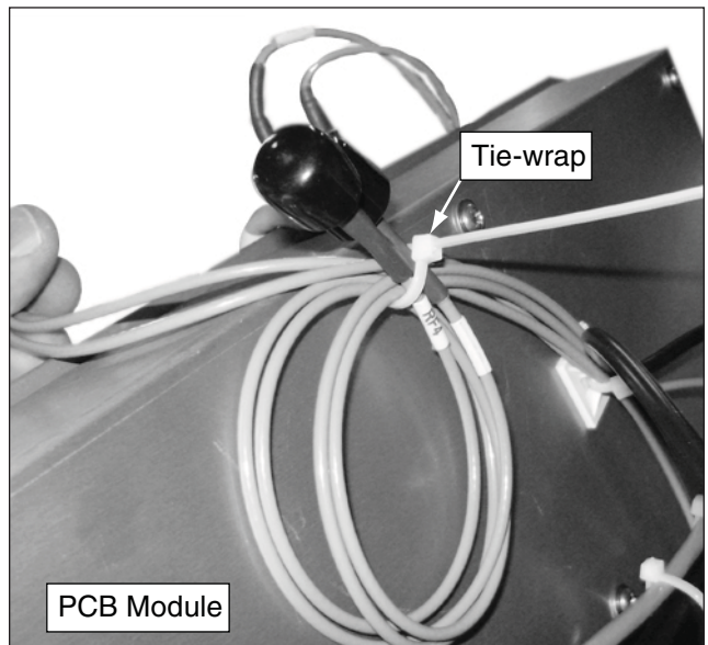
Figure 63 Excess Cable
