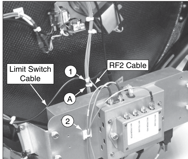
Figure 40 Tie-wrap Locations
