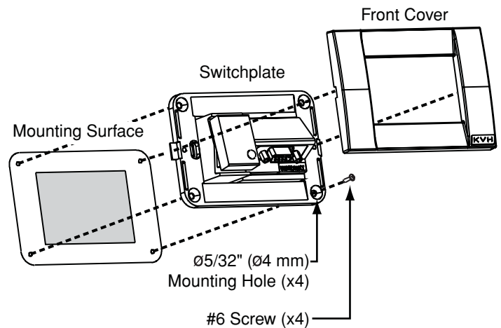
Figure 28: Mounting the Switchplate
