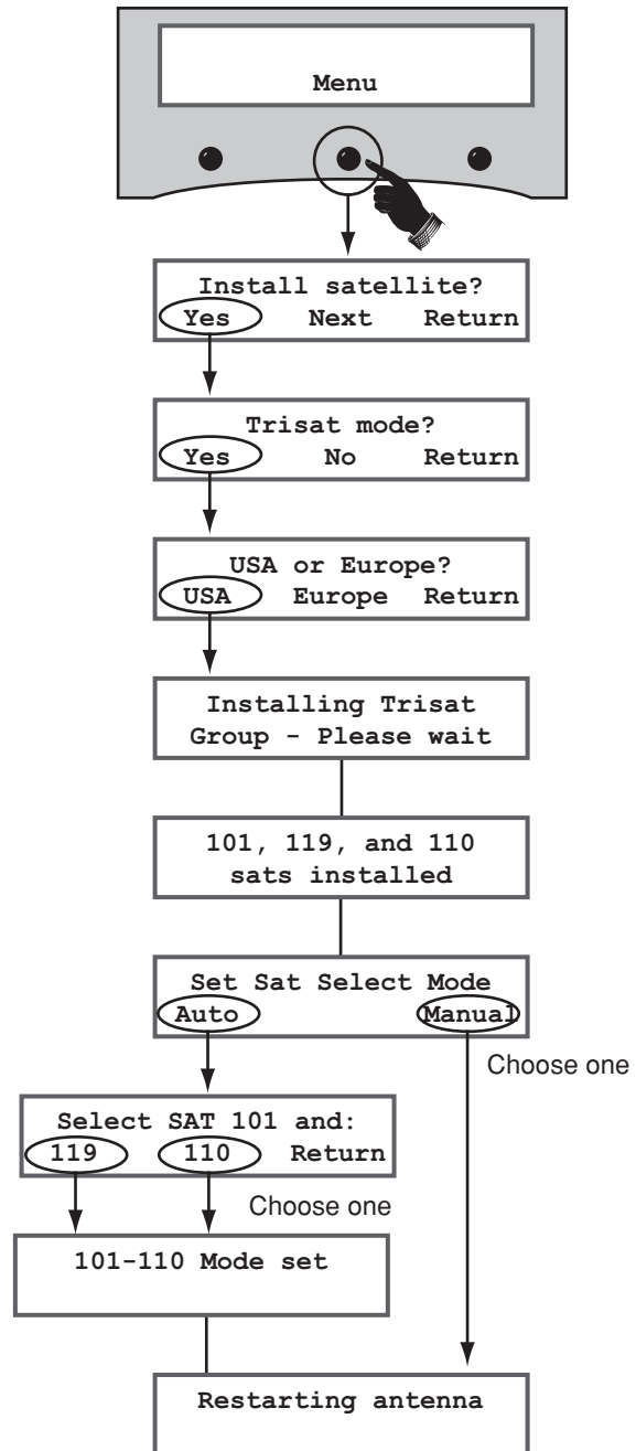
Figure 40: DIRECTV Trisat Group Selection Menus on MCP
