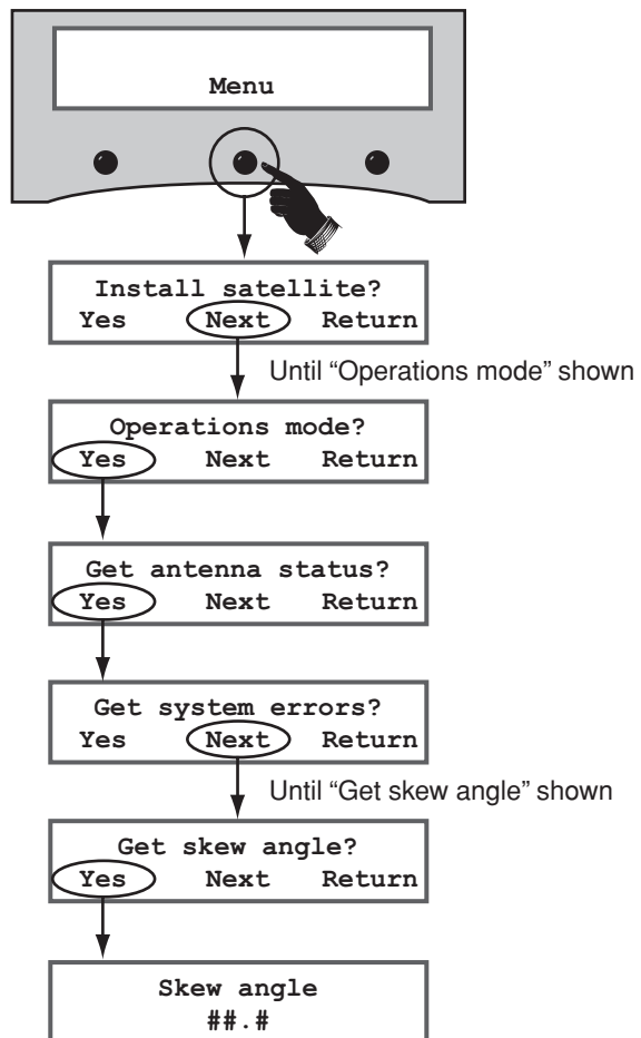
Figure 34: Skew Angle Menus on MCP
