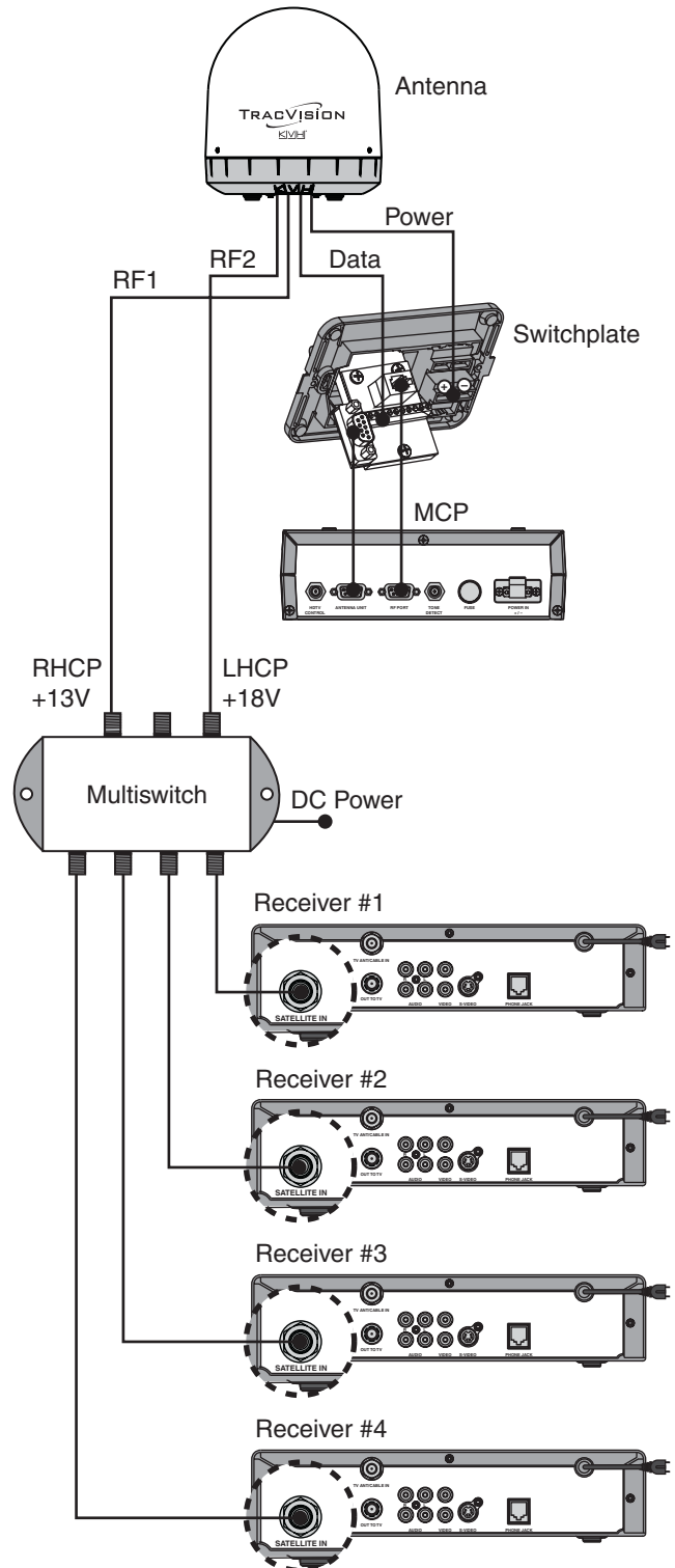
Figure 43: Multiswitch Wiring - Antenna with Circular Dual LNB
