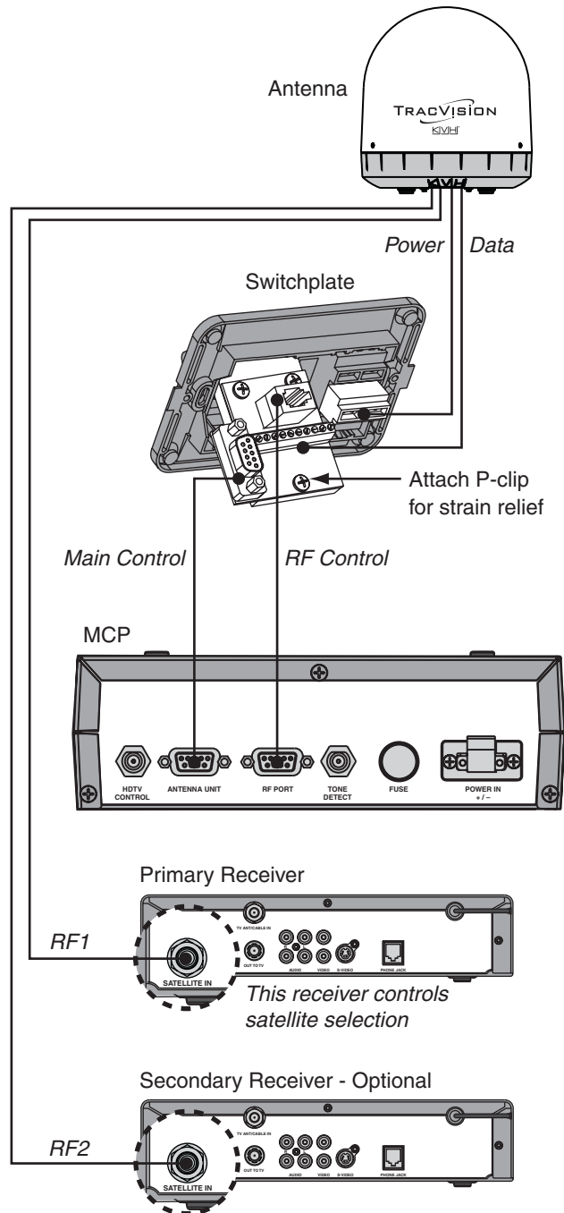
Figure 24: MCP and Receiver Wiring
