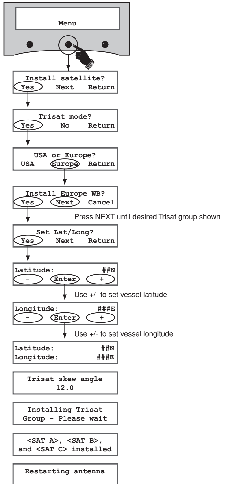
Figure 45: European Trisat Group Selection Menus on MCP
