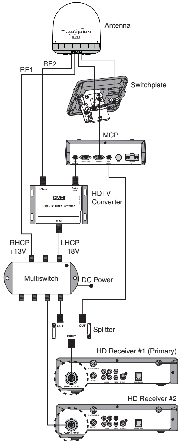
Figure 39: Wiring Multiple DIRECTV HD Receivers
