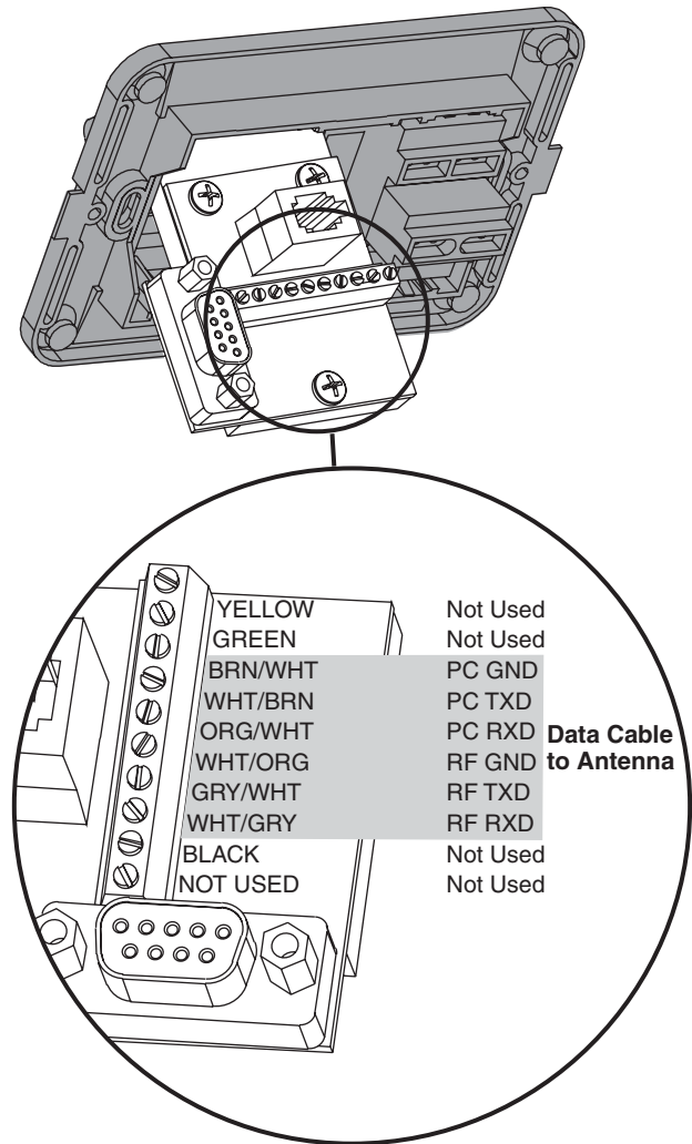
Figure 22: Switchplate Wiring - Antenna Data Cable
