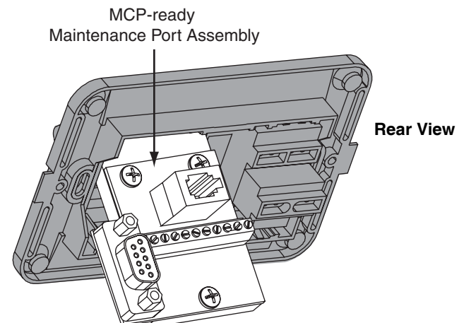
Figure 21: MCP-Ready Maintenance Port Assembly. Rear View.
