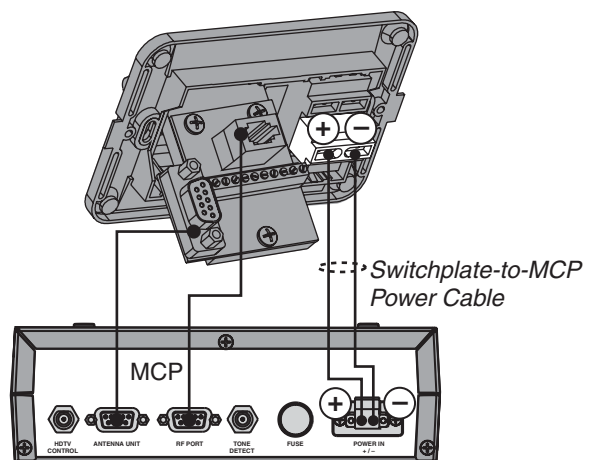
Figure 26: MCP Power Wiring
