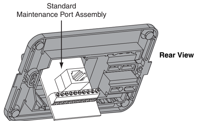
Figure 20: Standard Maintenance Port Assembly. Rear View.
