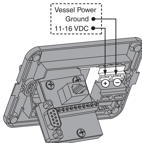
Figure 27: Switchplate Wiring - Vessel Power Cable
