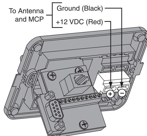
Figure 23: Switchplate Wiring - Antenna Power Cable
