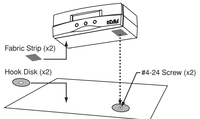
Figure 30: Flush Mounting the MCP to a Vertical Surface
