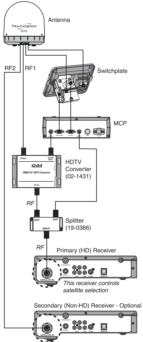
Figure 38: Wiring a Single DIRECTV HD Receiver
