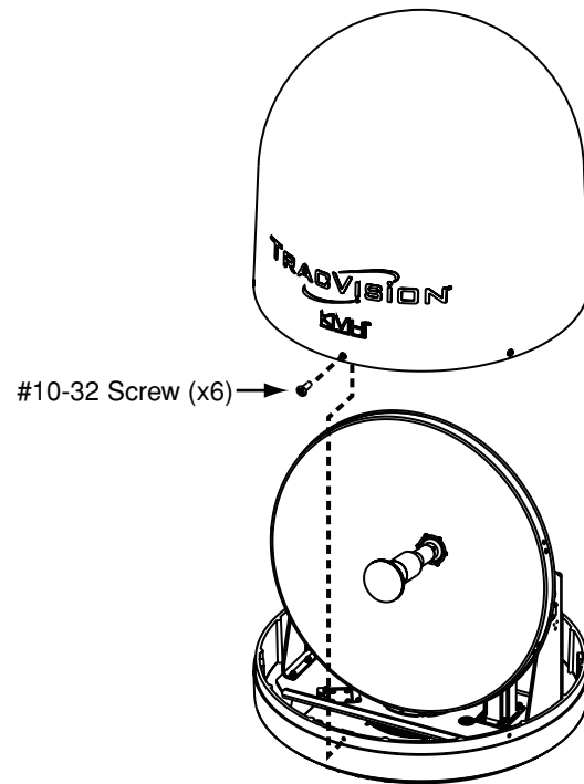
Figure 12: Removing the Radome
