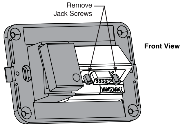
Figure 19: Detaching the Standard Maintenance Port Assembly
