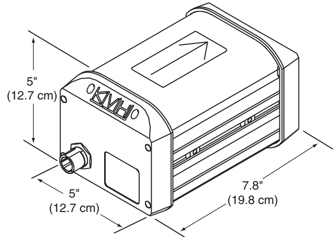
Figure 6: GyroTrac Sensor Dimensions
