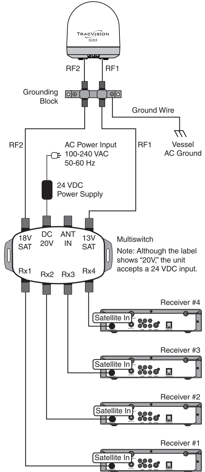
Figure 51: Multiswitch Wiring - Antenna with Circular Dual LNB
