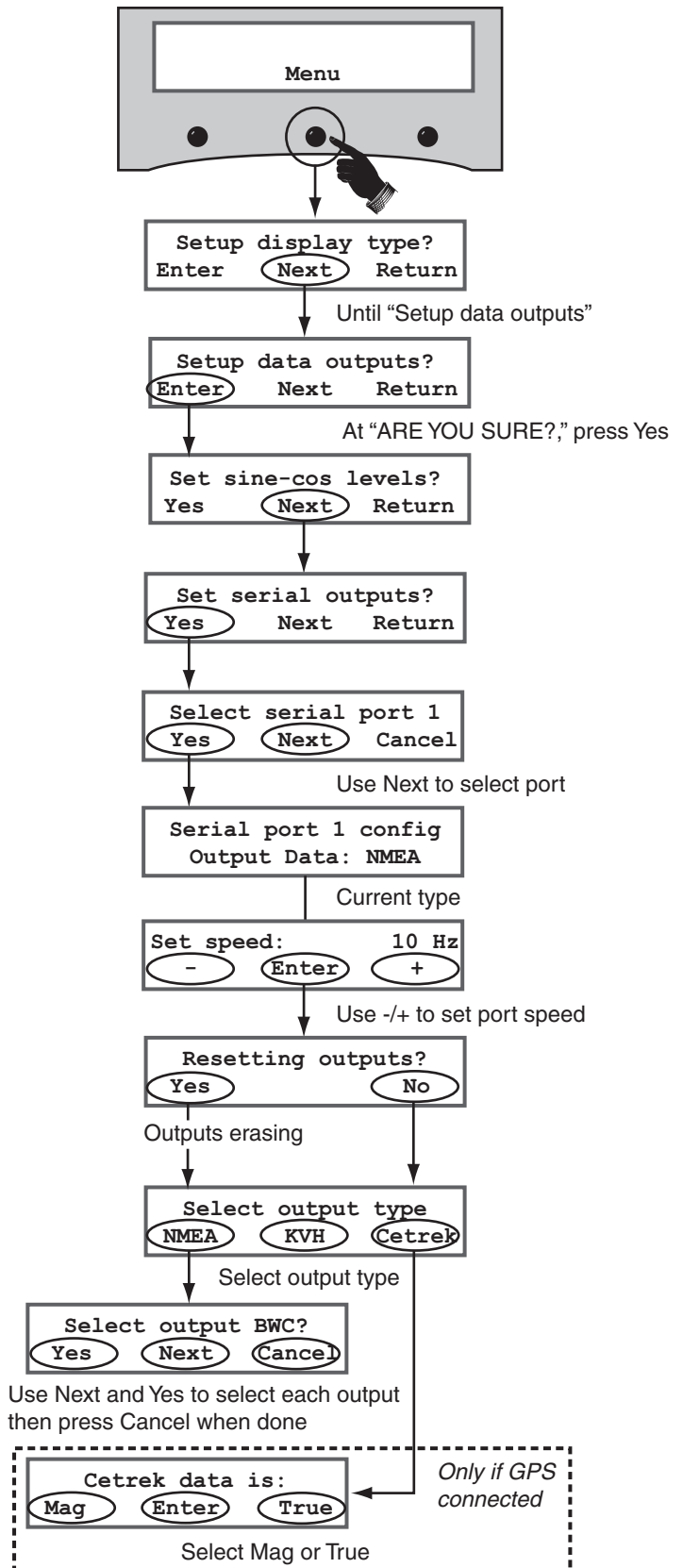
Figure 62: Serial Port Configuration Menus on ADCU
