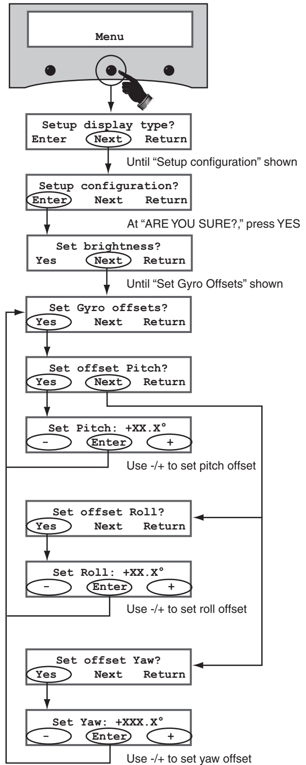
Figure 64: Gyro Offset Menus on ADCU
