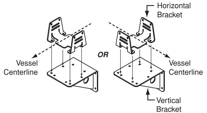
Figure 23: Bracket Mounting
