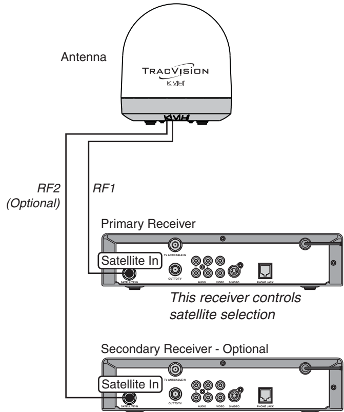
Figure 26: Wiring the Receivers to the Antenna
