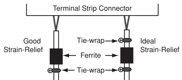
Figure 32: Effective Strain-Relief of ADCU Wires
