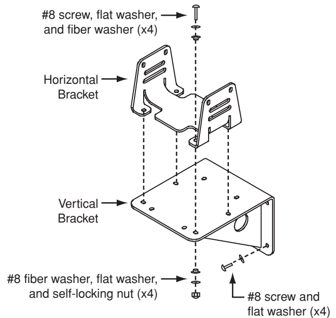
Figure 23: Bracket Mounting
