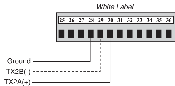
Figure 60: Serial Port #2 ADCU Wiring
