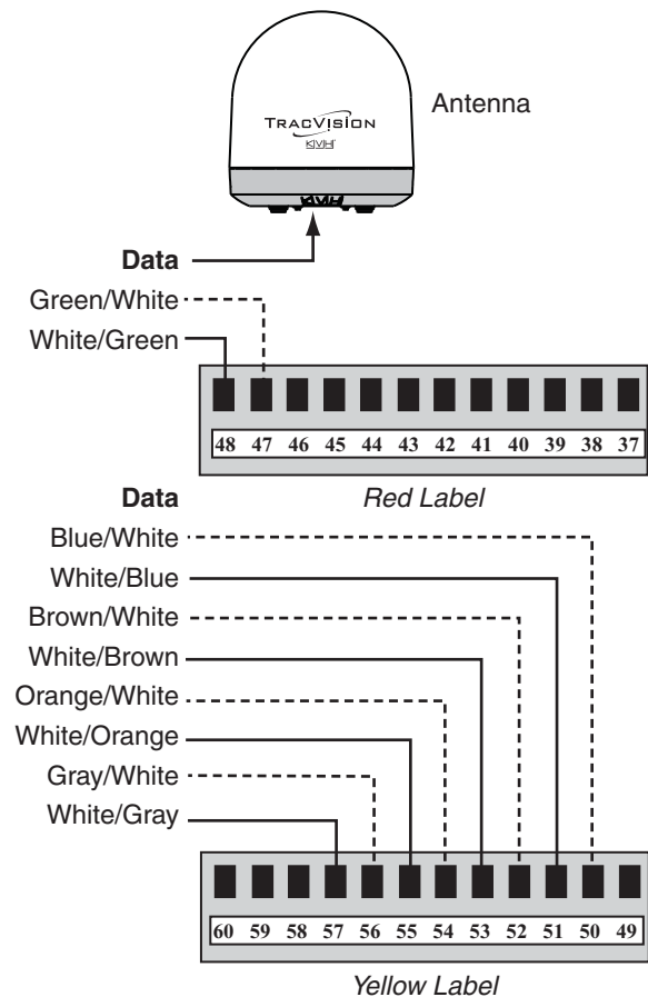
Figure 27: Wiring the Antenna to the ADCU
