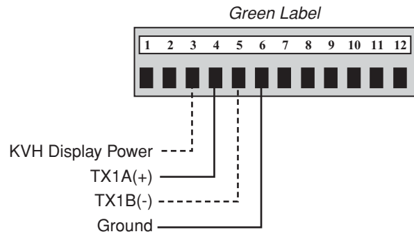
Figure 59: Serial Port #1 ADCU Wiring
