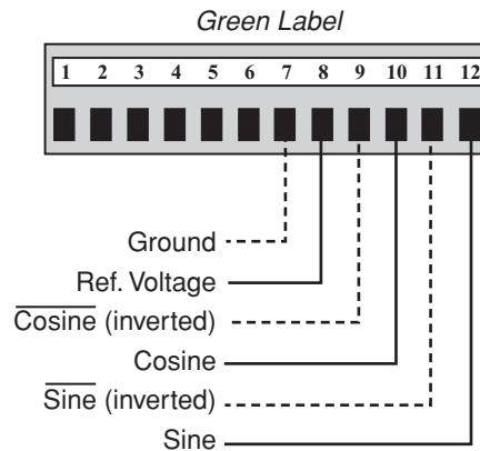
Figure 57: Sine/Cosine ADCU Wiring
