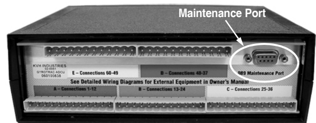
Figure 54: Maintenance Port on ADCU
