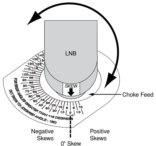
Figure 44: LNB Skew Angle Adjustment
