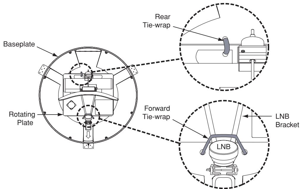
Tie-wrap Locations
