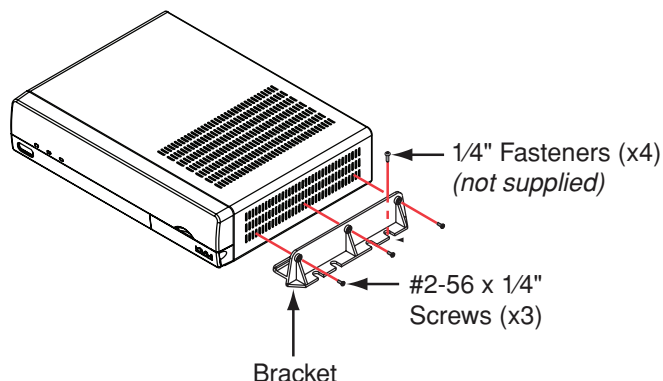
Figure 16 Receiver Brackets
