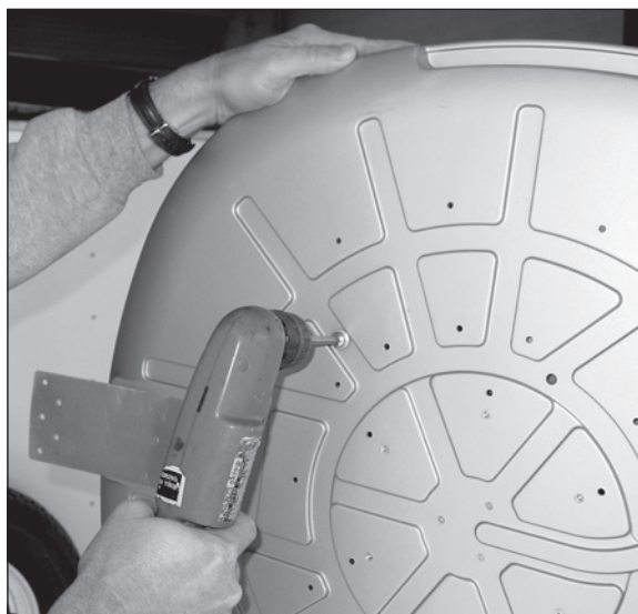
Figure 7 Removing the Shipping Restraints
