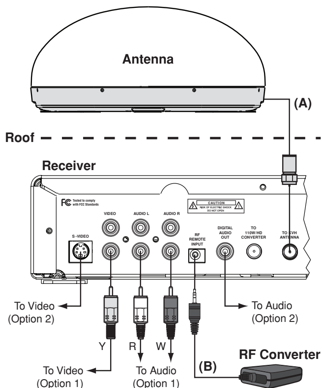
Figure 14 Receiver Wiring
