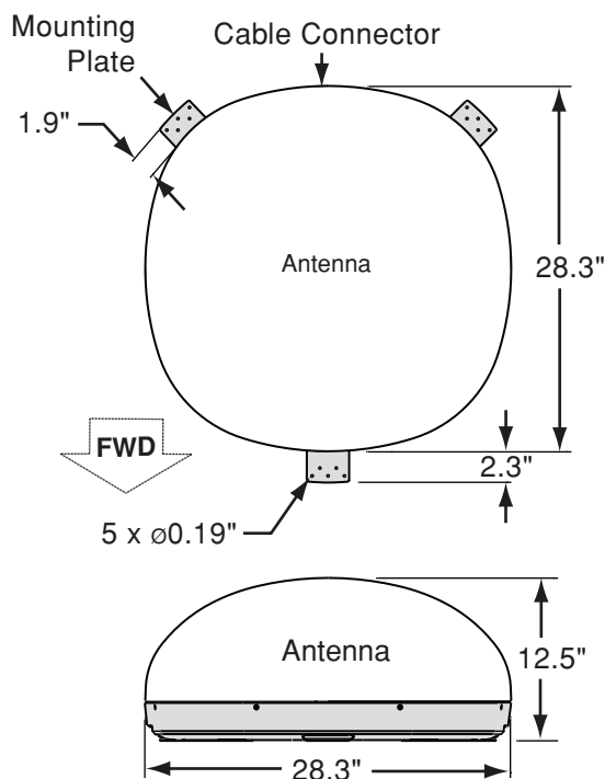
Figure 4 Antenna Dimensions
