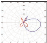
LED 28W Real light output - 1303 lm CRI > 80
