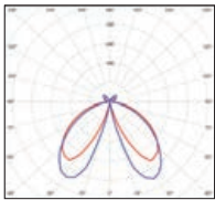
LED 20W Real light output - 743 lm CRI > 80
