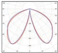
Models 1 to 11 except 4 LED 13W Real light output - 433 lm CRI > 80
