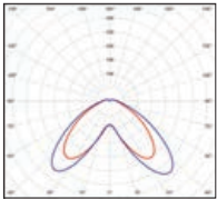
LED 35W Real light output - 2027 lm CRI > 80
