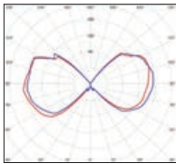
Models 3, 5 and 7 to 11 E27 (2450 lm) Real light output - 1659 lm
