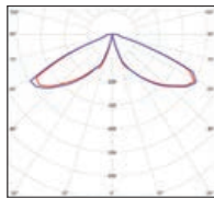
Models 1, 3, 9 E27 (2450 lm) Real light output - 506 lm
