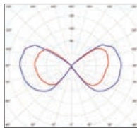
Models 4 to 8 and 10 to 12 E27 (2450 lm) Real light output - 1603 lm
