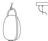
Kushi 33 suspension Ø 33 x H 56 Canopy Ø 12,5 x H 3
