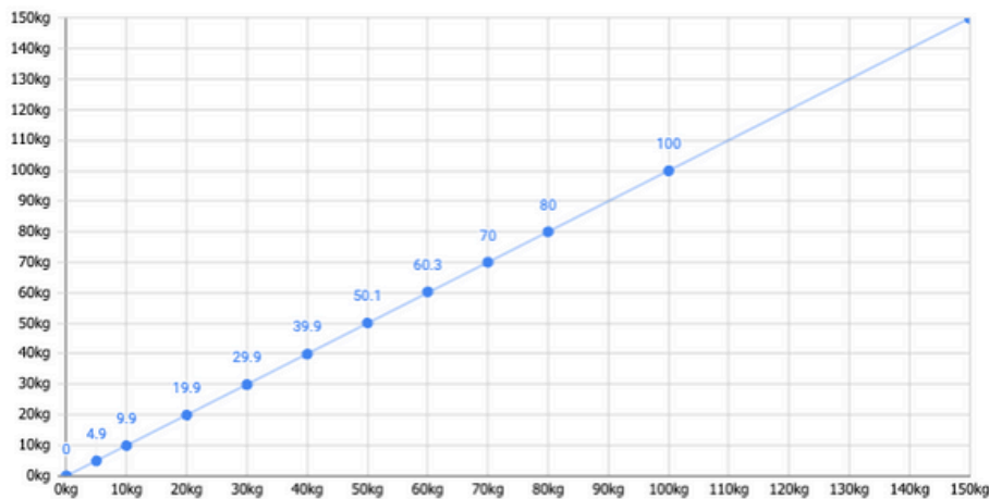
Gripper NATA Accreditation Testing - Tension
