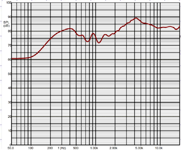
SPL-Response 4 ohm
