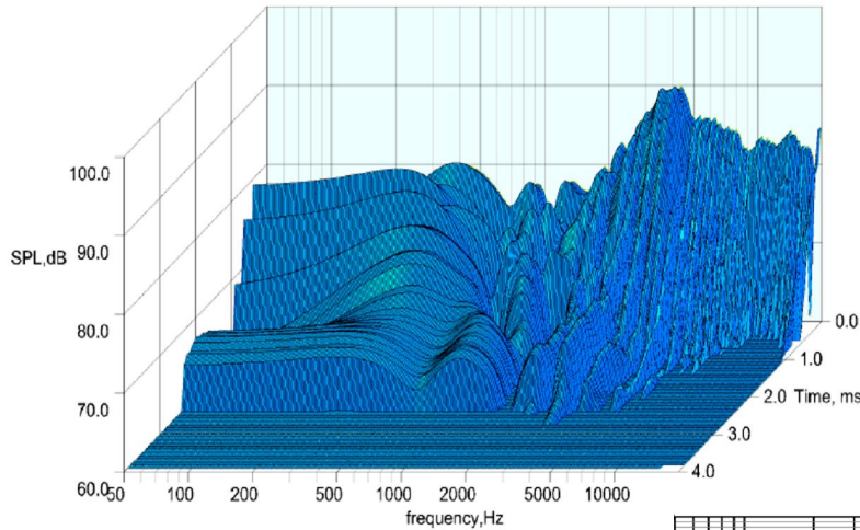
Waterfall Graph 4 ohm
