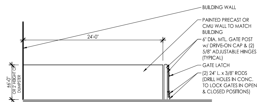
SIDE VIEW
