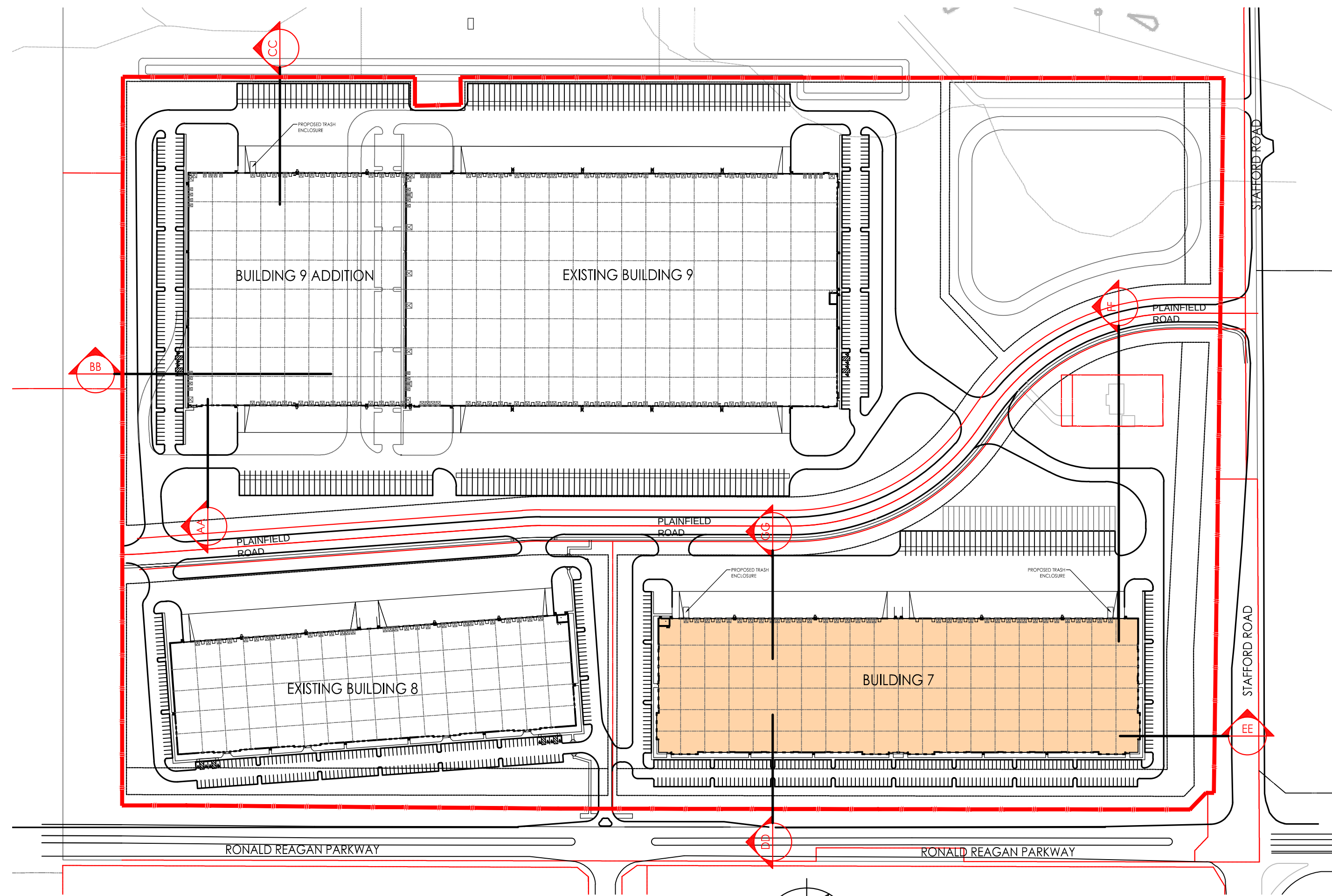
LOCATION PLAN 1" = 200'-0" 0 50 100 200 400'
