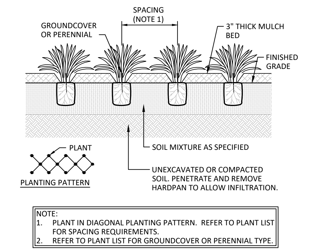
3 GROUNDCOVER / PERENNIAL PLANTING DETAIL NO SCALE
