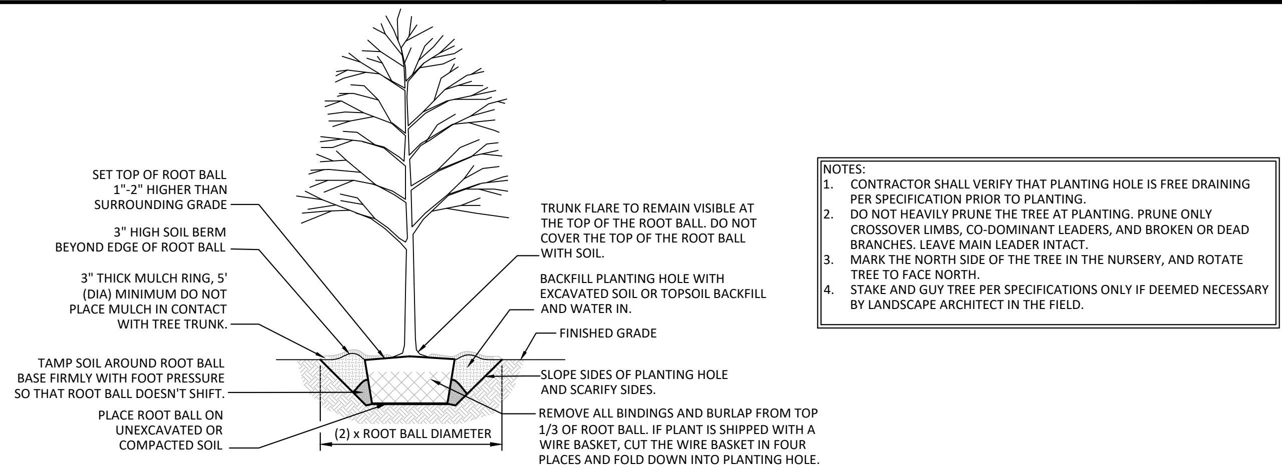
1 DECIDUOUS TREE PLANTING DETAIL NO SCALE
