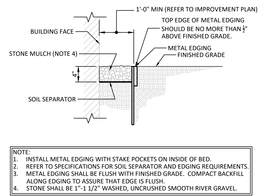
6 STONE MULCH DETAIL NO SCALE
