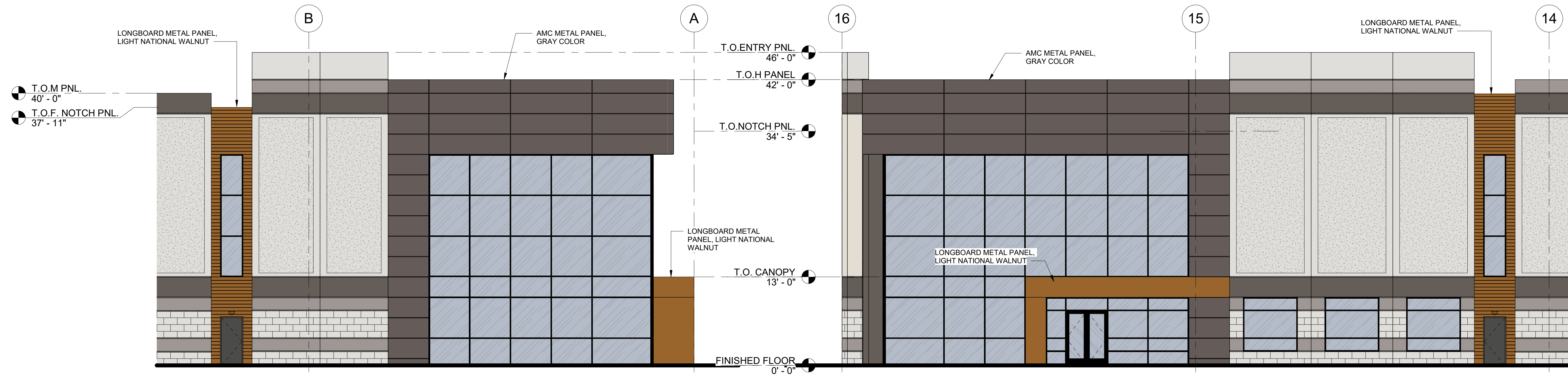
2 ENLARGED NORTHWEST CORNER A201 1/8" = 1'-0"
