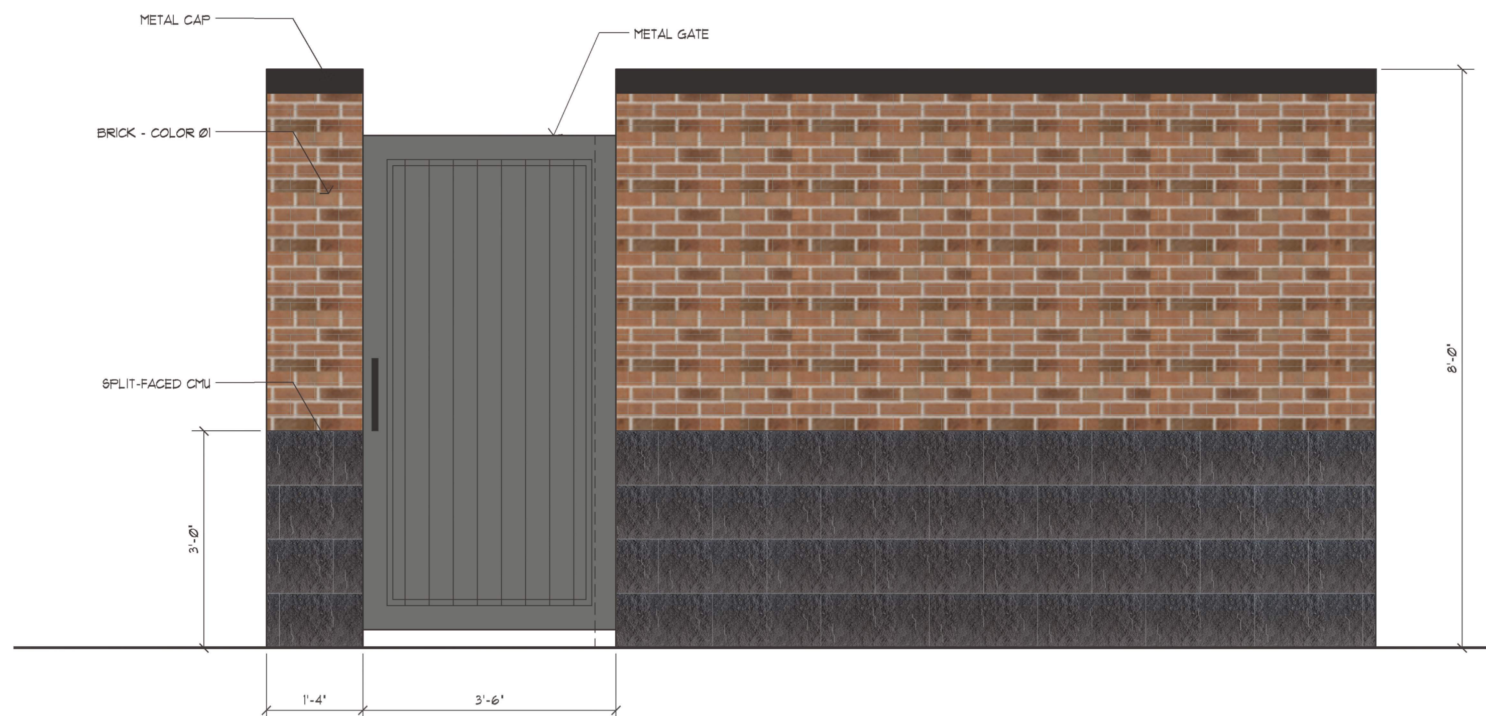
○ REAR ELEVATION SCALE: 3/4"=1'-0"
