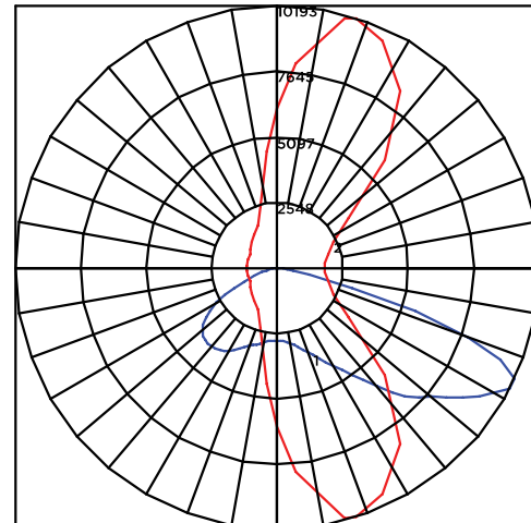
POLAR CURVE
