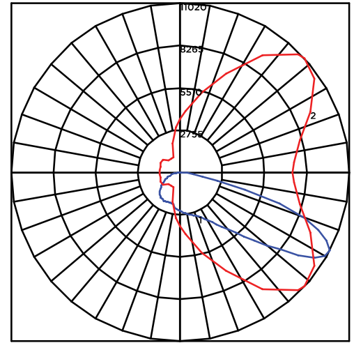
POLAR CURVE
