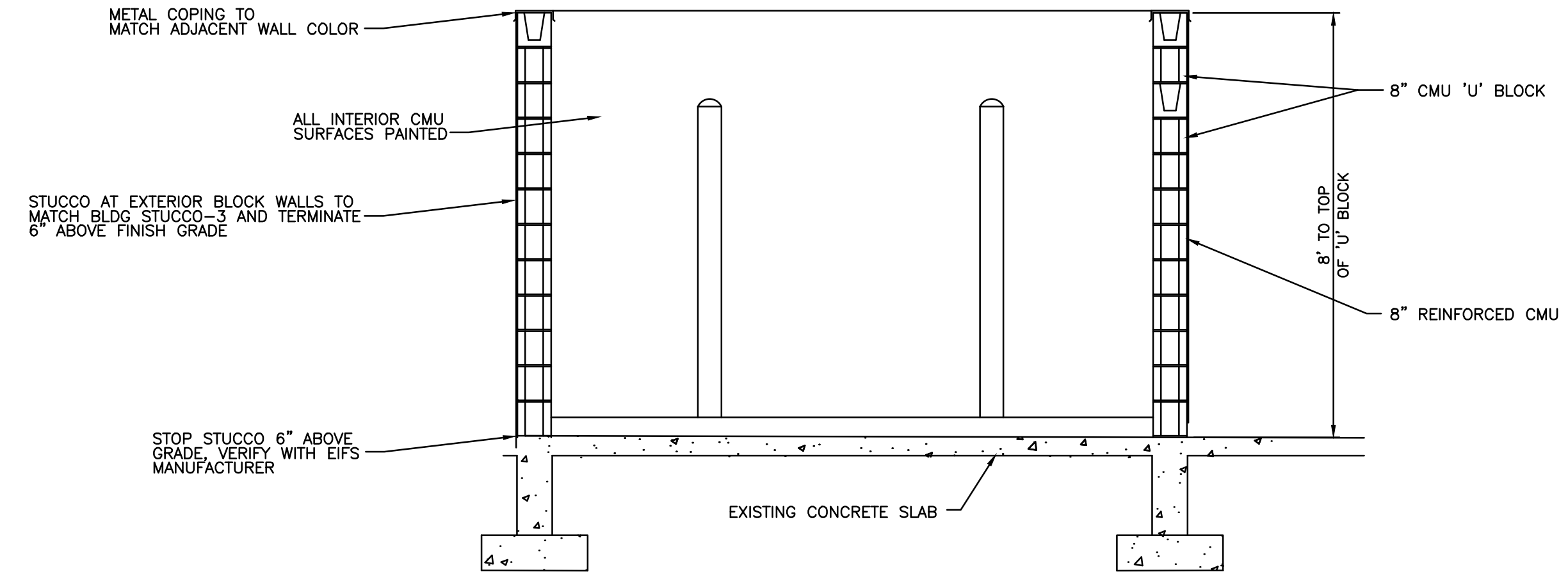
DUMPSTER ENCLOSURE
