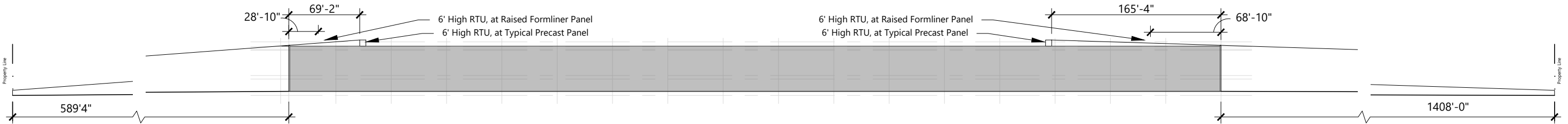
Section D
