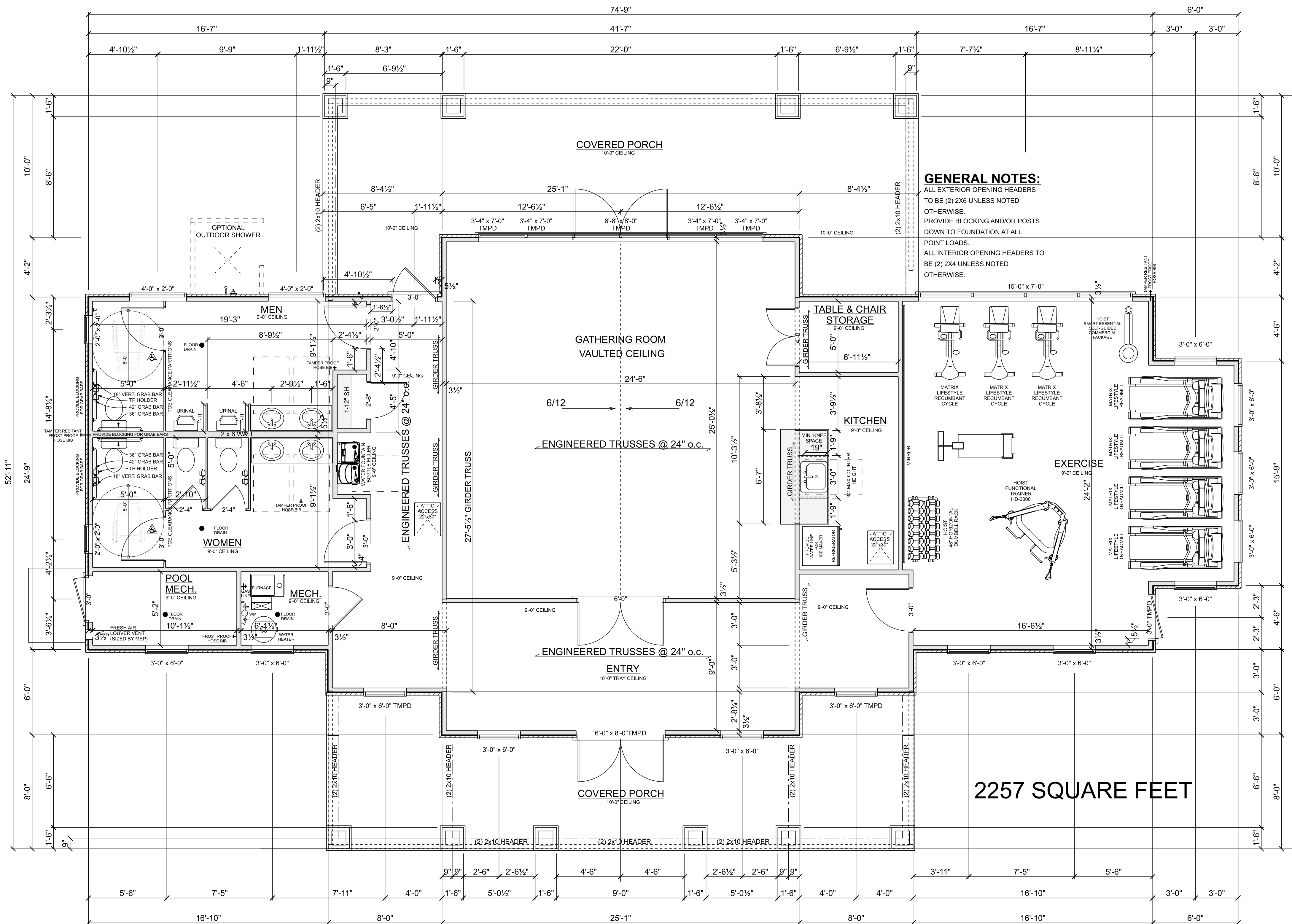
2.1 BoMar Clubhouse Floor Plan SCALE: 1/4" = 1'-0"
