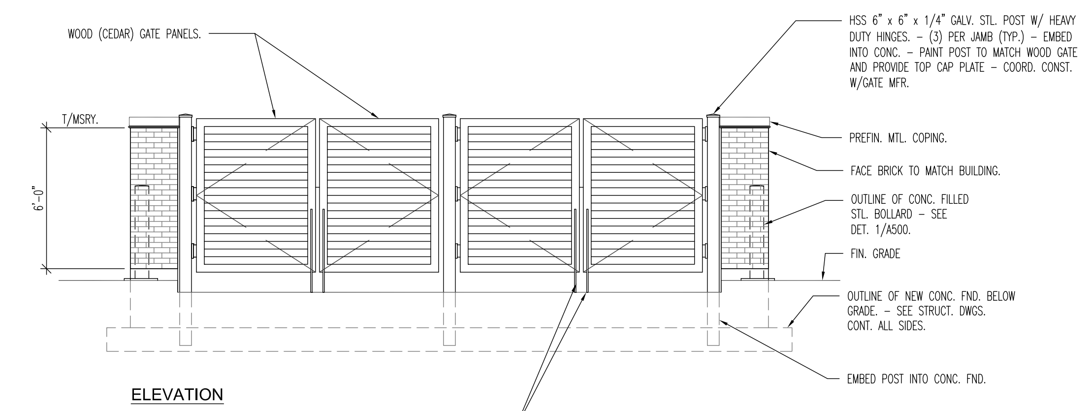
1 DETAIL SCALE: 1/4" = 1'-0" DUMPSTER ENCLOSURE
