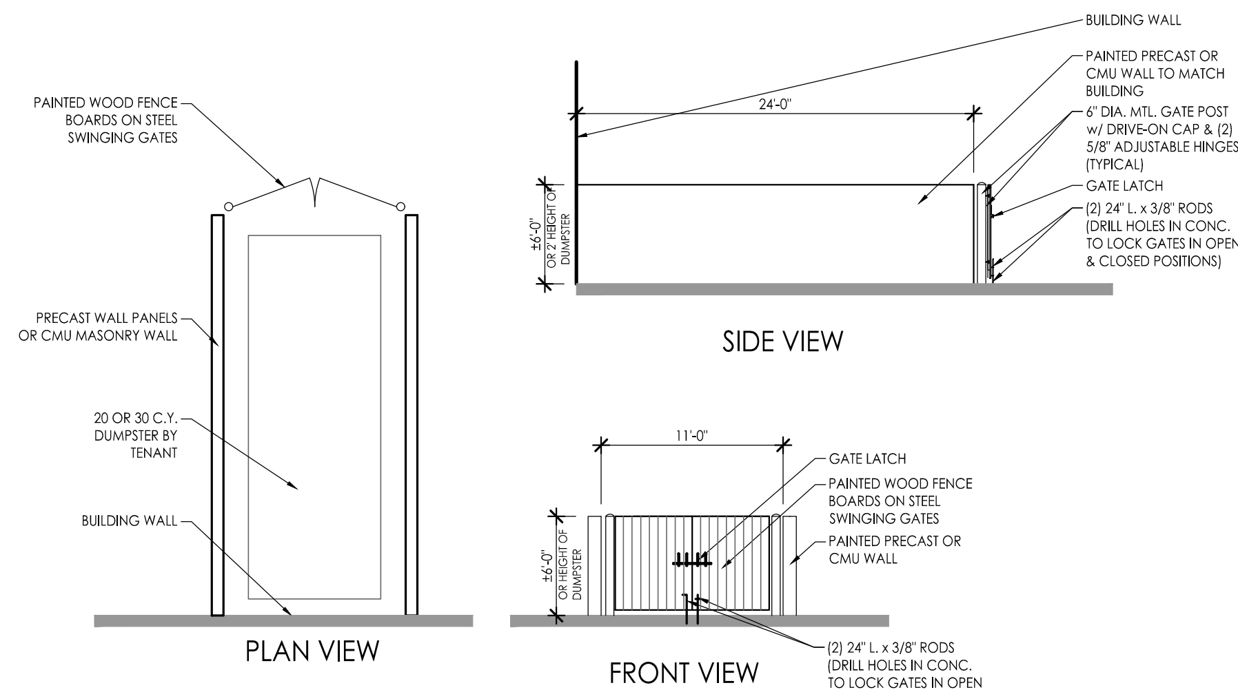
TRASH ENCLOSURE
