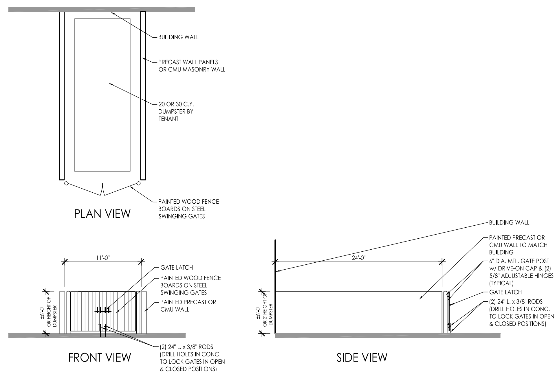
DUMPSTER ENCLOSURE 1/8" = 1'-0" 0 2' 4' 6' 16'
