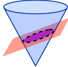
Ellipse
