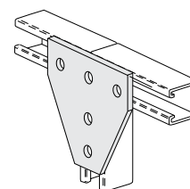
TEE GUSSET PLATE 5065 3-Hole 5075 4-Hole 5080 5-Hole (Shown) 5085 6-Hole
