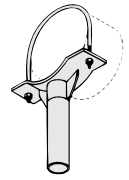
Fig. 882 Pipe Saddle Support with U-Bolt
