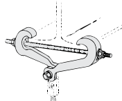
Fig. 630 Malleable Center Load Beam Clamp
