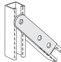
SWIVEL PLATE 5020 2-Hole 5023 3-Hole (Shown)
