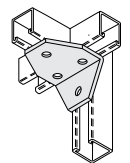
JOINT ANGLE CONNECTOR 5200 4-Hole (Shown) 5205 5-Hole
