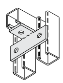
5148 3-Hole Offset Bent Tee
