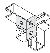
5140-5146 3-Hole Offset Bent Angle 5140 & 5145 (Shown)
