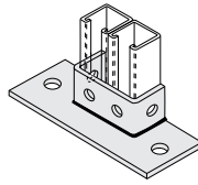
6045 Post Base for Double 1 5 / 8 Struts
