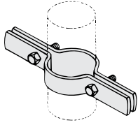
Fig. 552 & 554 Copper Tubing Riser Clamp
