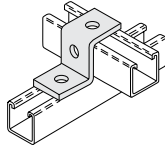
"Z" SUPPORT 5551 2-Hole for #1200 Strut 5552 3-Hole for #1500 Strut 5553 2-Hole for #1600 Strut 5554 3-Hole for #1000 Strut (Shown)
