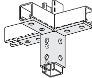
TRIPLE WING CONNECTOR 5650 6-Hole 5655 12-Hole (Shown) 5660 9-Hole
