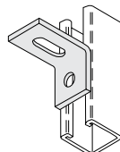
5220-5226 2-Hole Adjustable Corner Angle 5221 (Shown)
