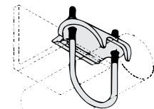
Fig. 840 Right Angle Clamp
