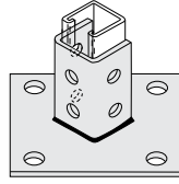
6020 Post Base for 1 5 / 8 Struts
