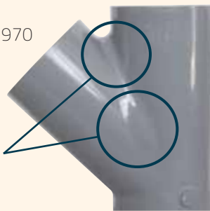
Gusset and Reinforced Wye Branch
