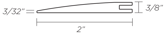
3/8" Flush Reducer
