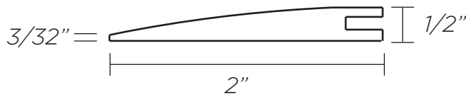
1/2" Flush Reducer
