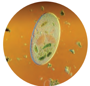
Figure 2.33 This paramecium has ingested (eaten) two smaller organisms, called euglena. The green euglena are visible inside the paramecium near the bottom of the micrograph. Through the process of digestion, the paramecium extracts sugars produced in the chloroplasts of the euglena and provides them to its own mitochondria for energy production.
