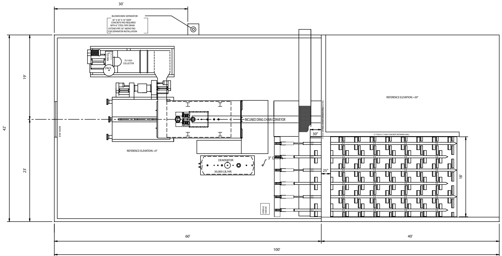
PLAN VIEW
