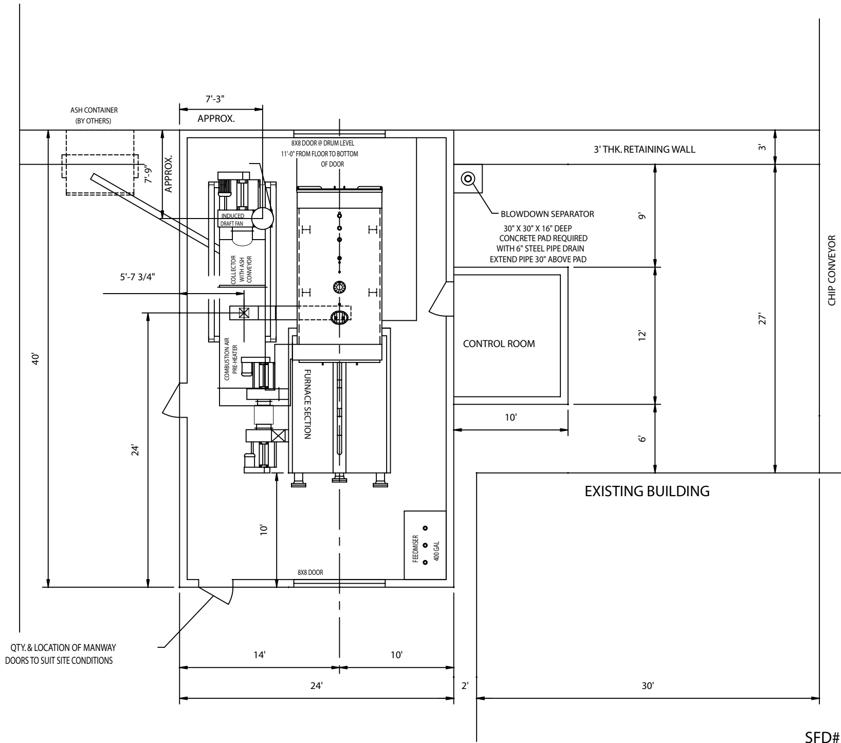
PLAN VIEW
