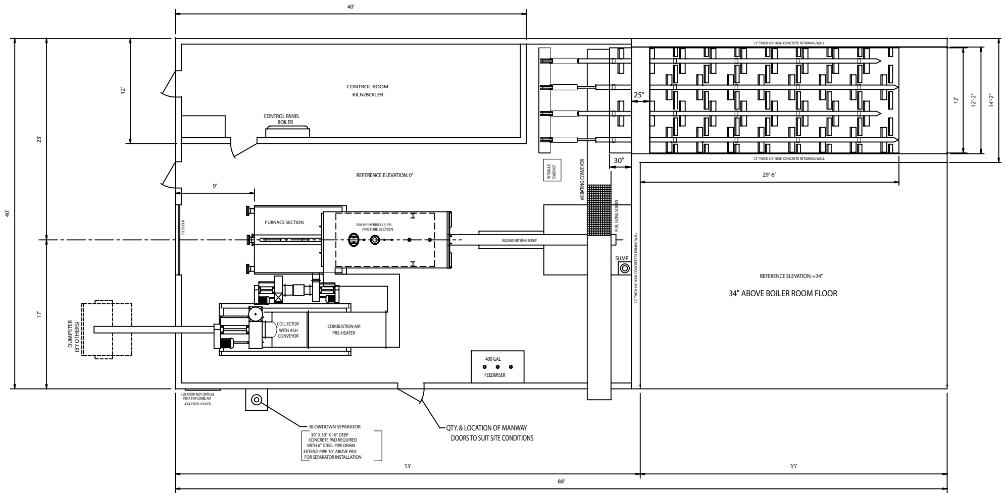
PLAN VIEW
