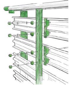
Shock absorbers Anti-vandalism caps
