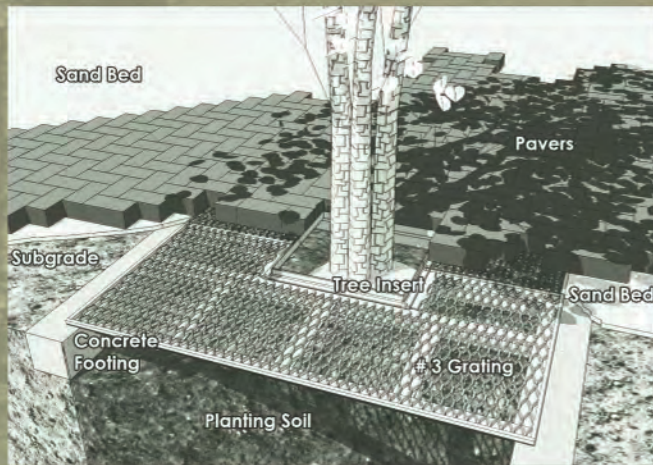
Paver-Grate™ with Market Street trim ring in cast aluminum
